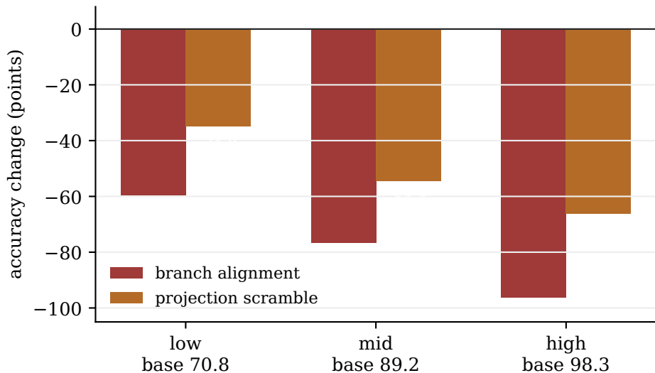
Statistic-preserving scrambles destroy ICL
