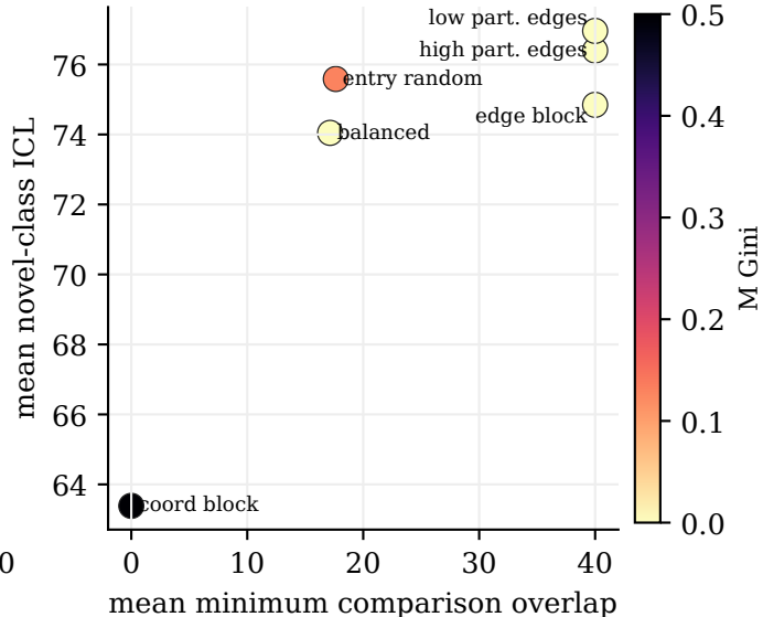
Branch overlap is the direct risk variable
