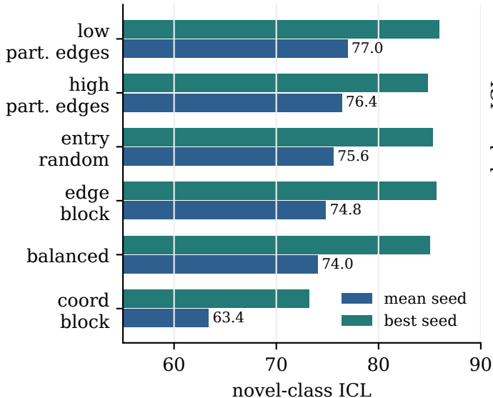
Mask family changes ICL at fixed count
