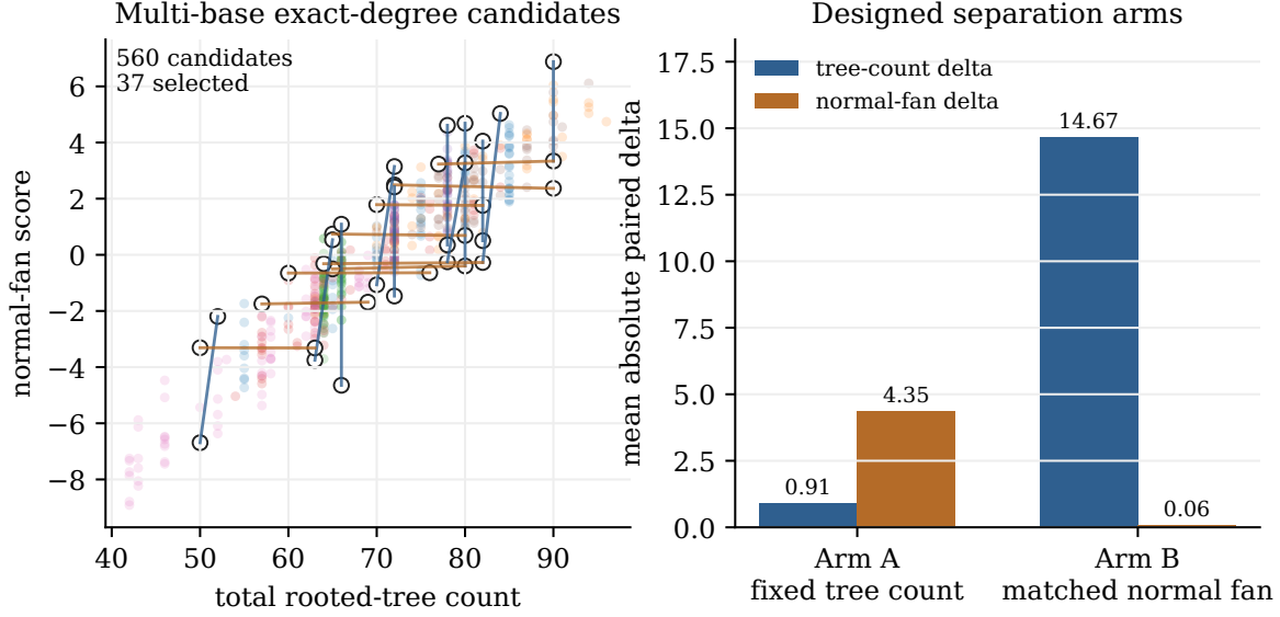
Figure 16: Multi-base exact-control design. Arm A holds rooted-tree count nearly fixed while varying normal-fan score. Arm B varies rooted-tree count while matching normal-fan score.
