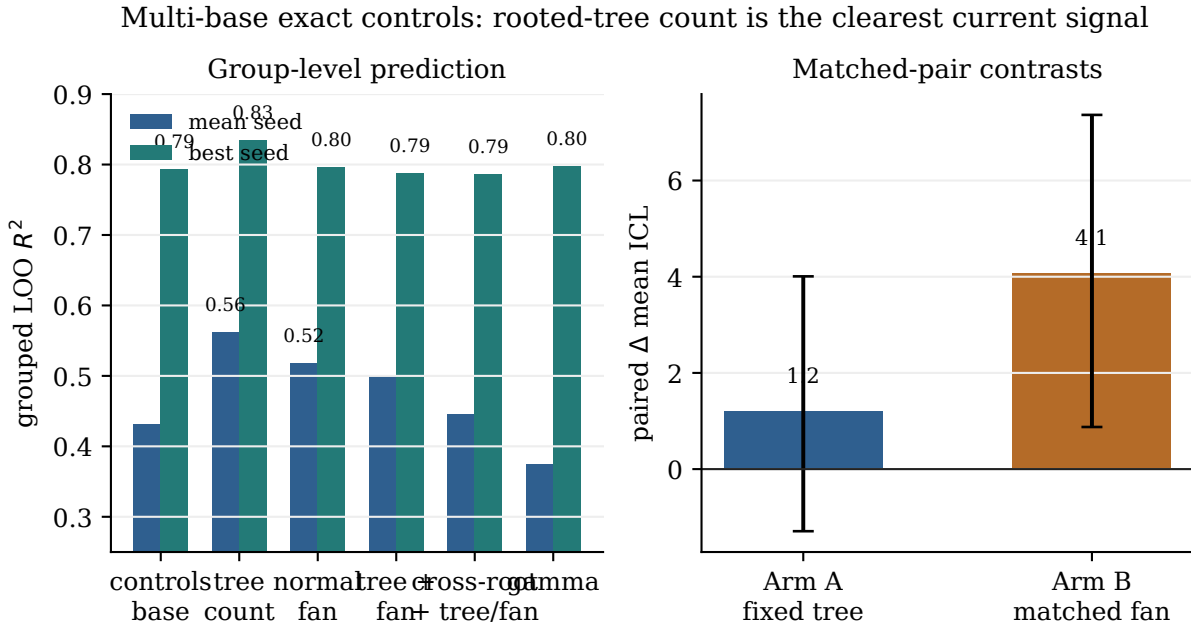
Figure 17: Completed multi-base exact-control analysis. Tree count plus base controls gives the best grouped LOO prediction. The matched-pair contrast is clearer for Arm B, where tree count varies at matched normal-fan score.
