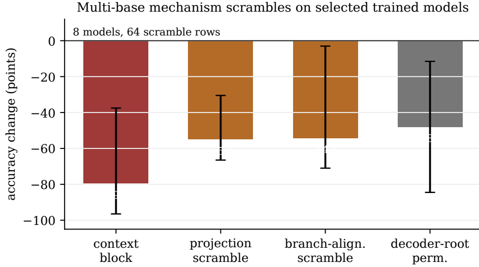
Figure 18: Multi-base mechanism follow-up. Even when pre-training predictors remain imperfect, trained high-performing models depend causally on branch/projection/tree organization.
