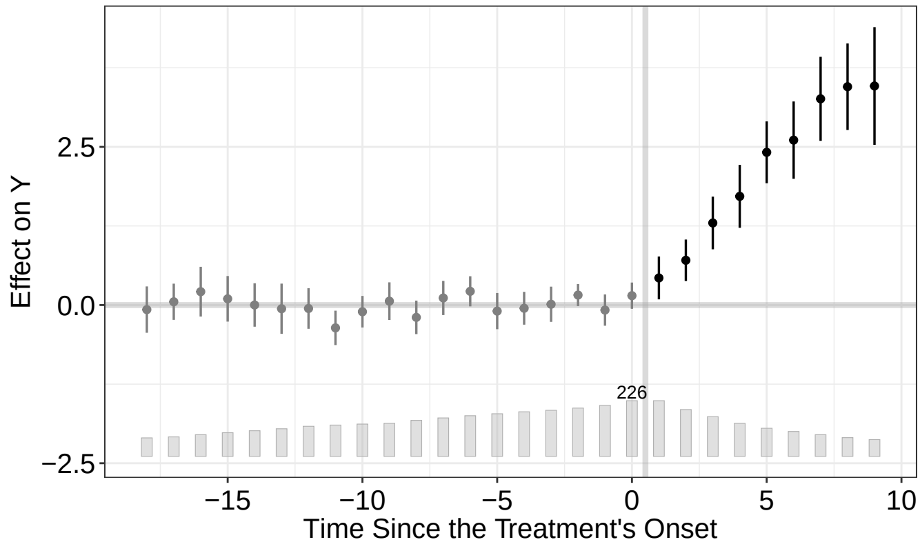
fect: ATT with 95% CI (IFE, r = 2 )
