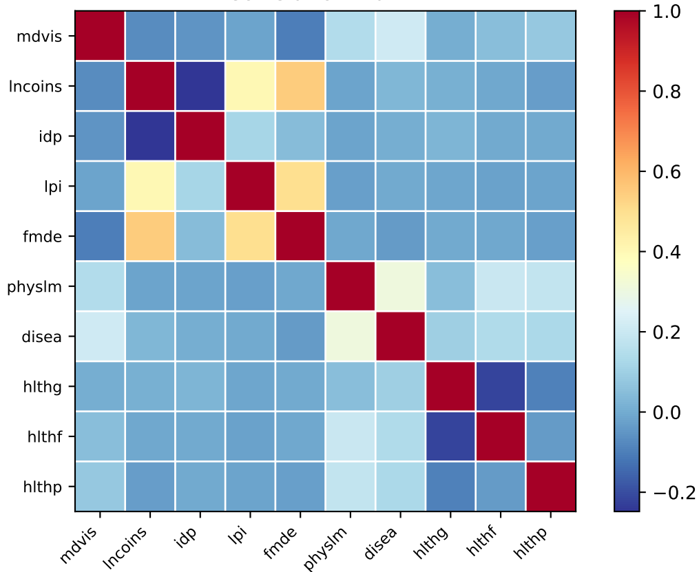
Correlation Matrix
