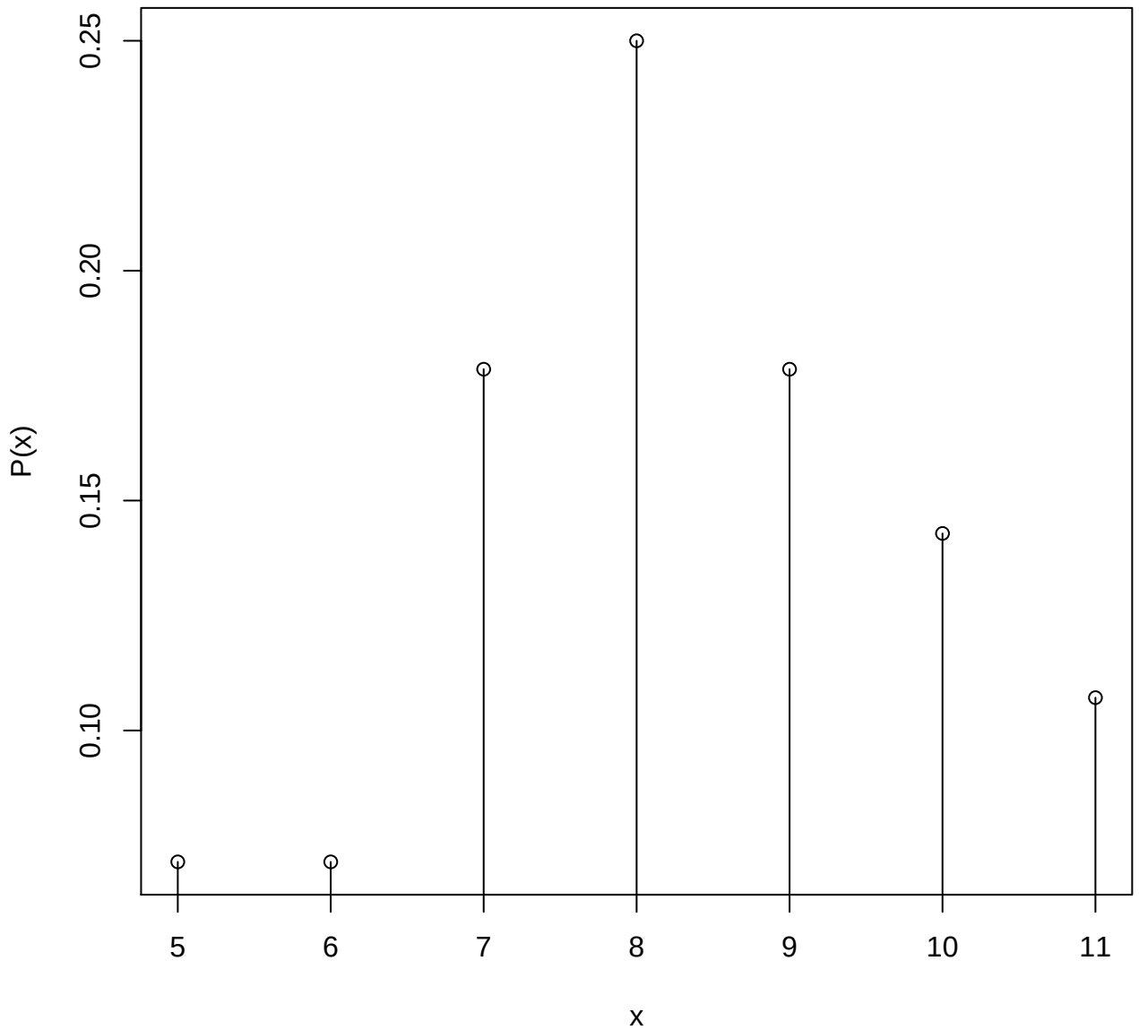
Probability Distribution for M & M Data
