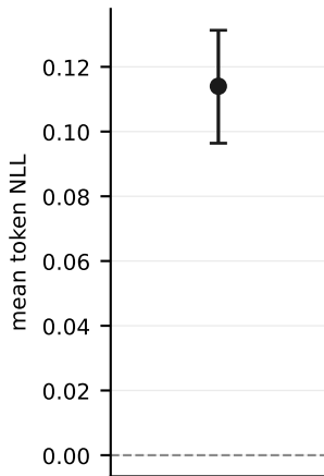
3. zero-shot nll-v2
