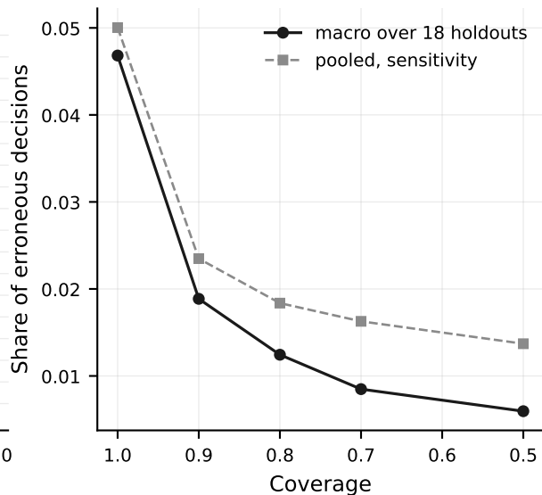
Risk-coverage: no threshold selected
