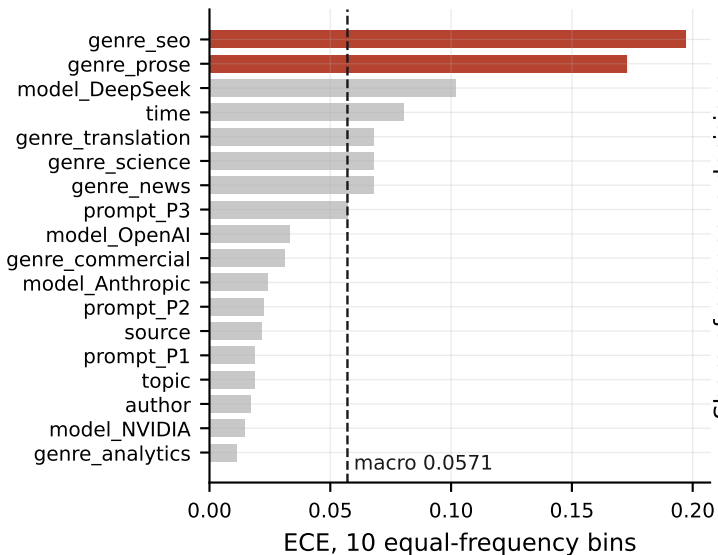
Calibration is heterogeneous
