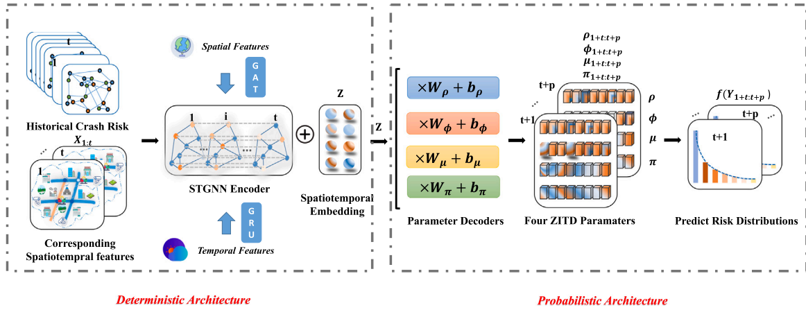
Fig. 2. The overall framework of STZITD-GNNs. STZITD-GNNs utilise the ST-GNN Encoder \mathcal{ST} (composed of GRU and GAT encoders) to encode the history time window 1:t crash risk Y_{1:t} , and road features X_{1:t} with the use of the road connection graph in the spatial-temporal embedding of the road \mathcal{Z} . After encoding, the four parameter decoders map \mathcal{Z} into the ZITD parameter space and obtain \pi_{t+1:t+p}, \mu_{t+1:t+p}, \phi_{t+1:t+p}, \rho_{t+1:t+p} for the predicted time window t+1:t+p , which determine the predicted road traffic crash risk distribution f(Y_{t+1:t+p}) . Note: This figure is a simplified representation. For a complete list of features, including weather and road characteristics, please refer to Table 3.
