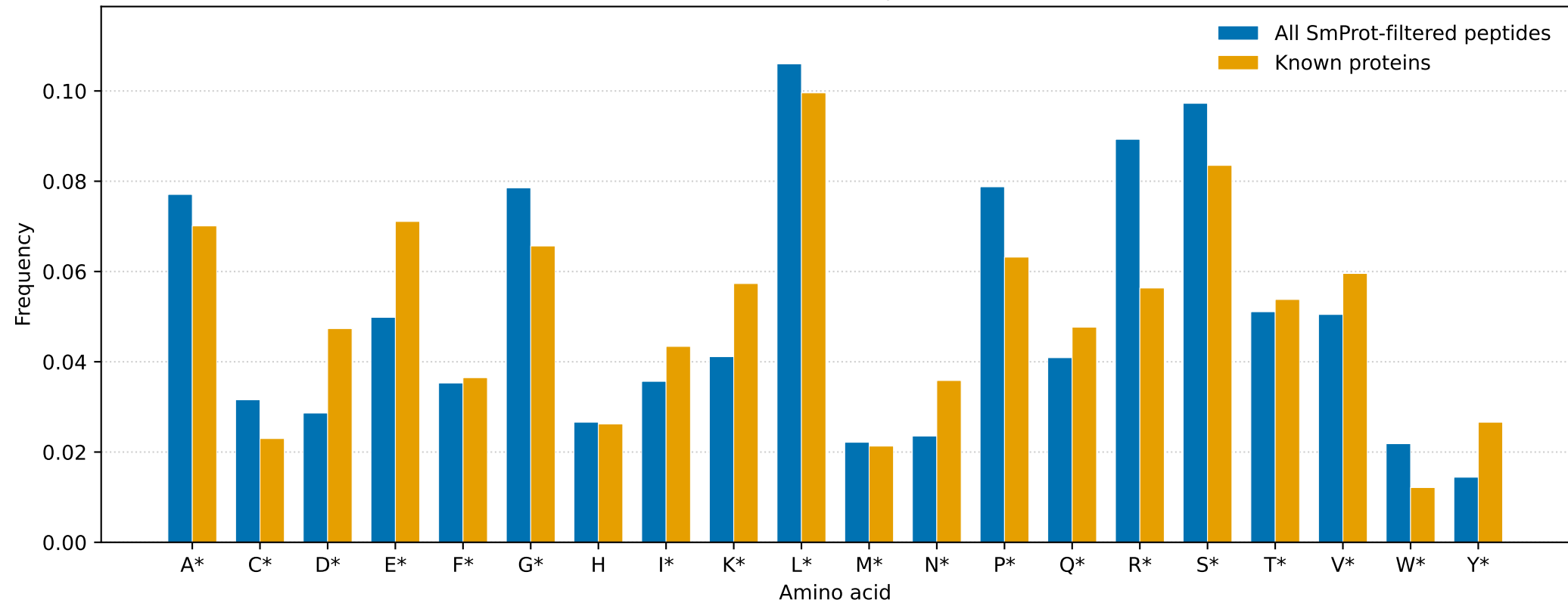
Amino acid frequency comparison All SmProt-filtered peptides: 118,091 AAs | Known proteins: 11,413,722 AAs
