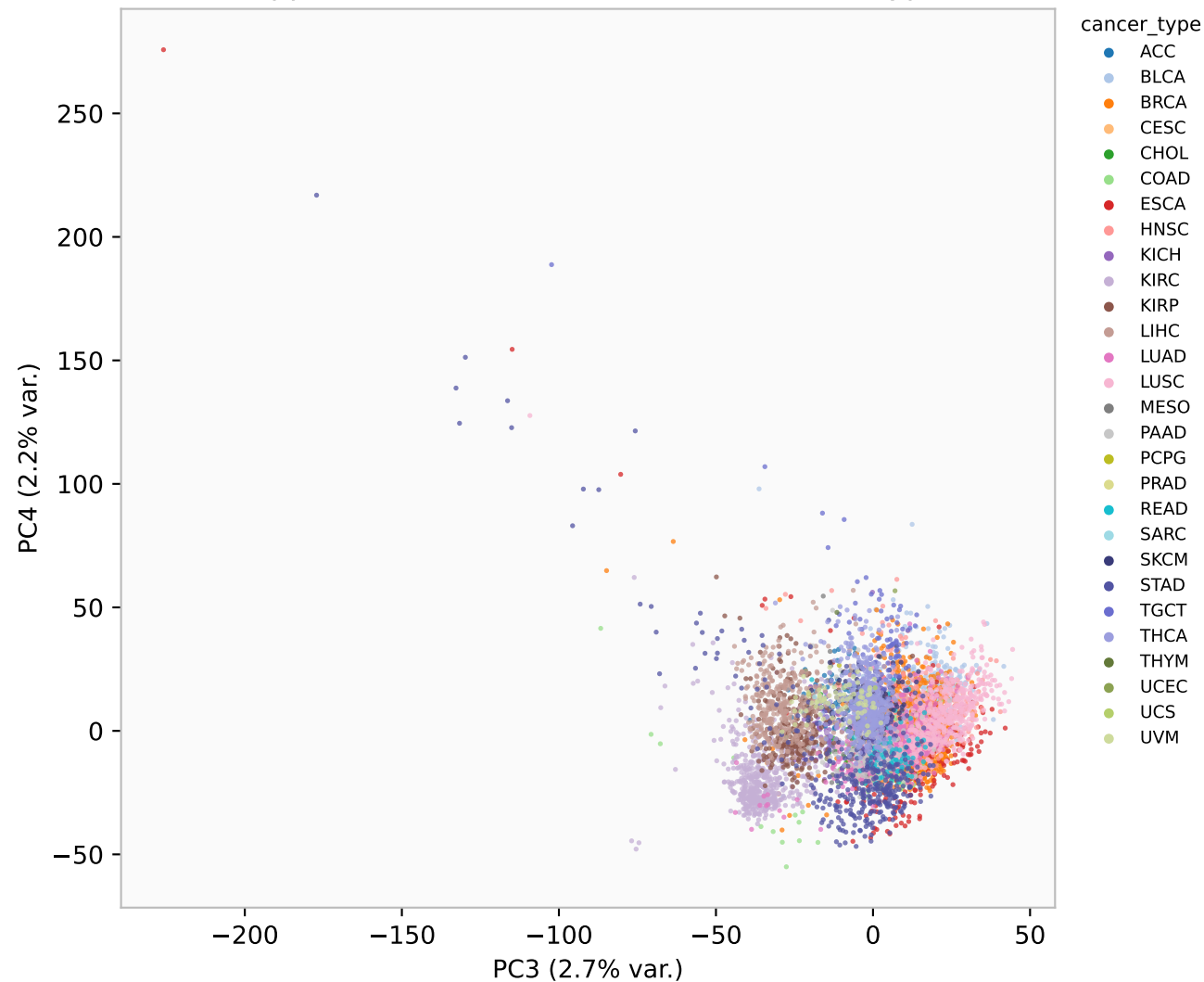
Supplement — PCA (PC3 vs PC4) — cancer type
