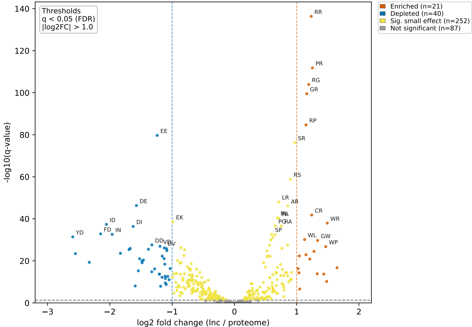
Volcano plot: 2-mer enrichment (lncRNA peptides (TCGA-matrix) vs proteome)
