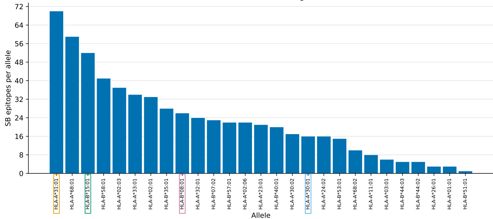
Per-allele SB load (Tr-lncRNA-MPs, merged IEDB+NetMHC)
