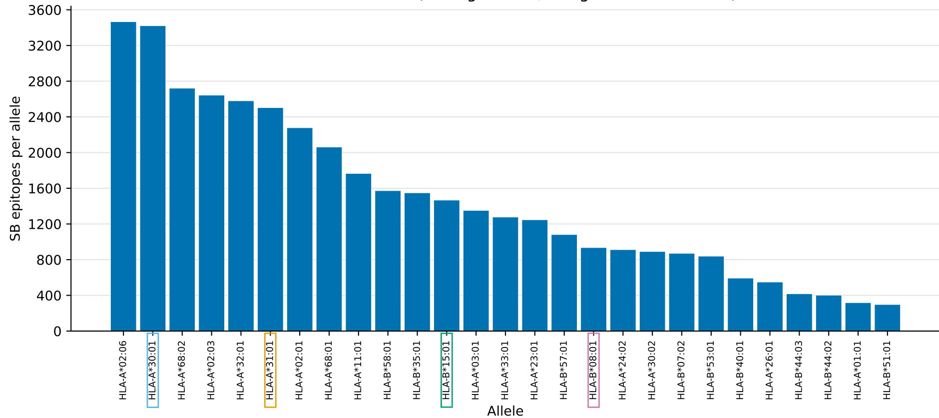
Per-allele SB load (coding control, merged IEDB+NetMHC)
