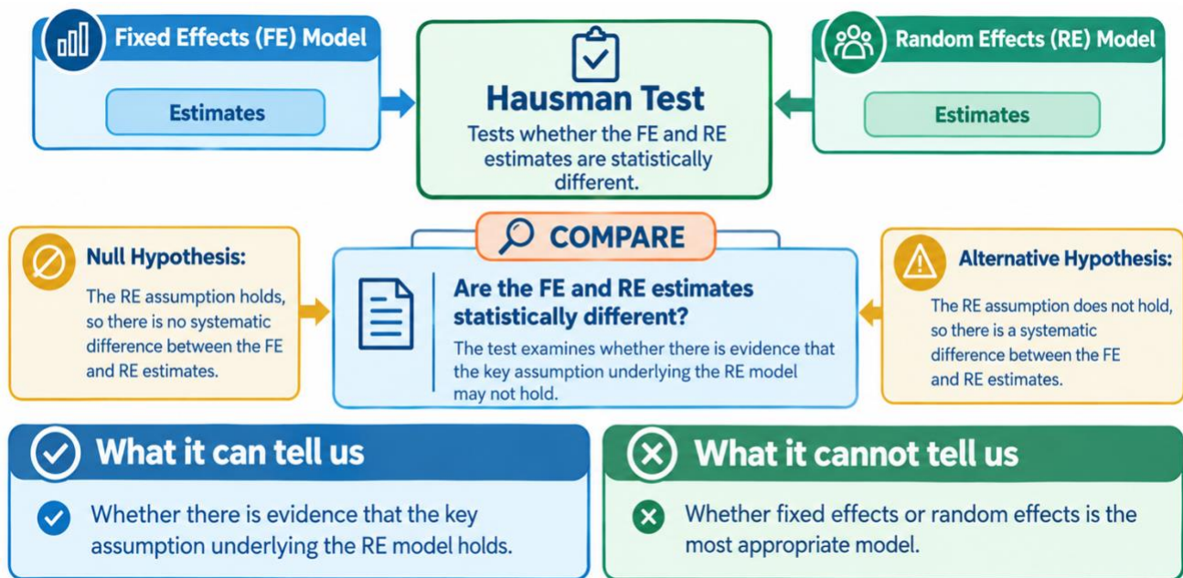
Figure 2: The Hausman Test: The Logic Behind It
