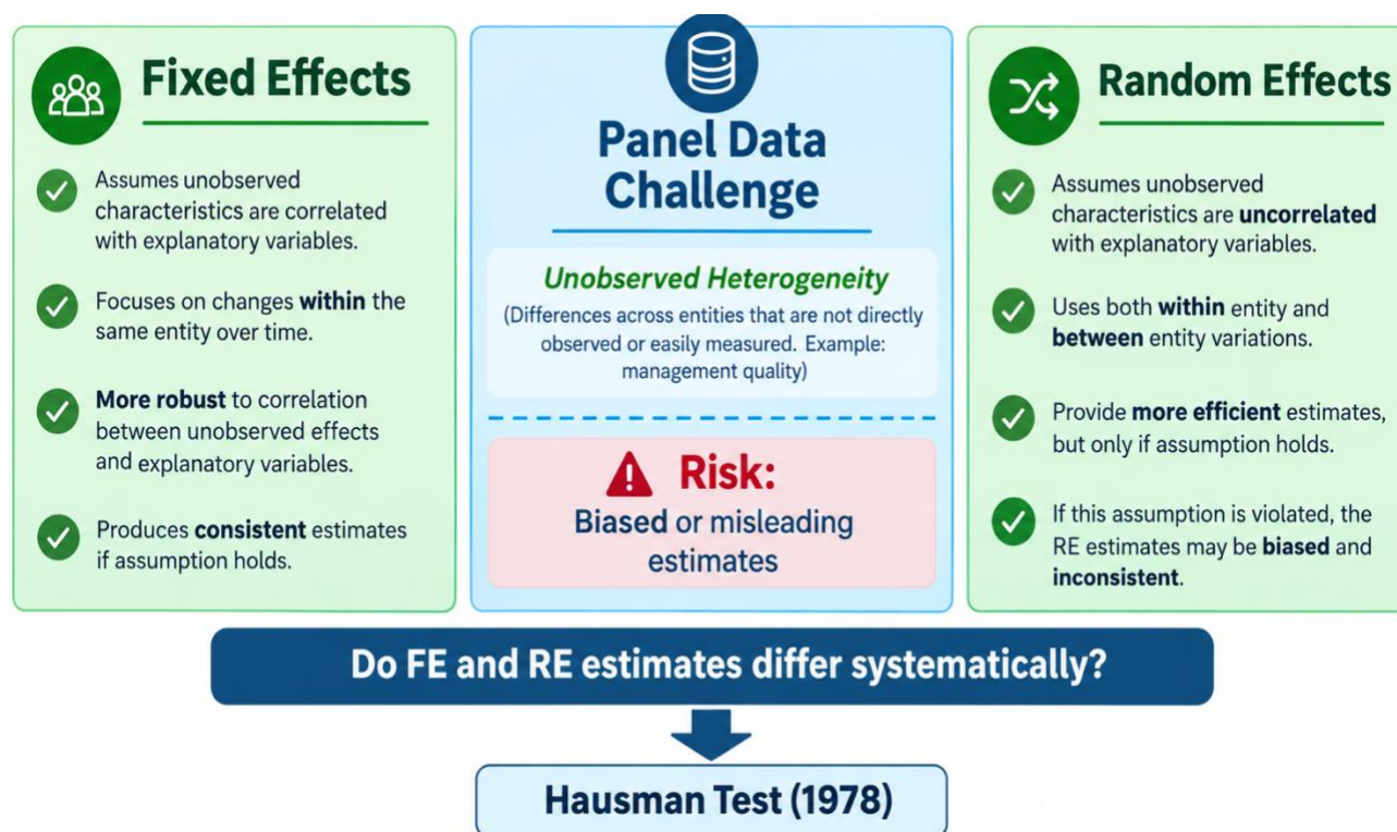
Figure 1: The Fixed Effects Model - Random Effects Model Trade Off
