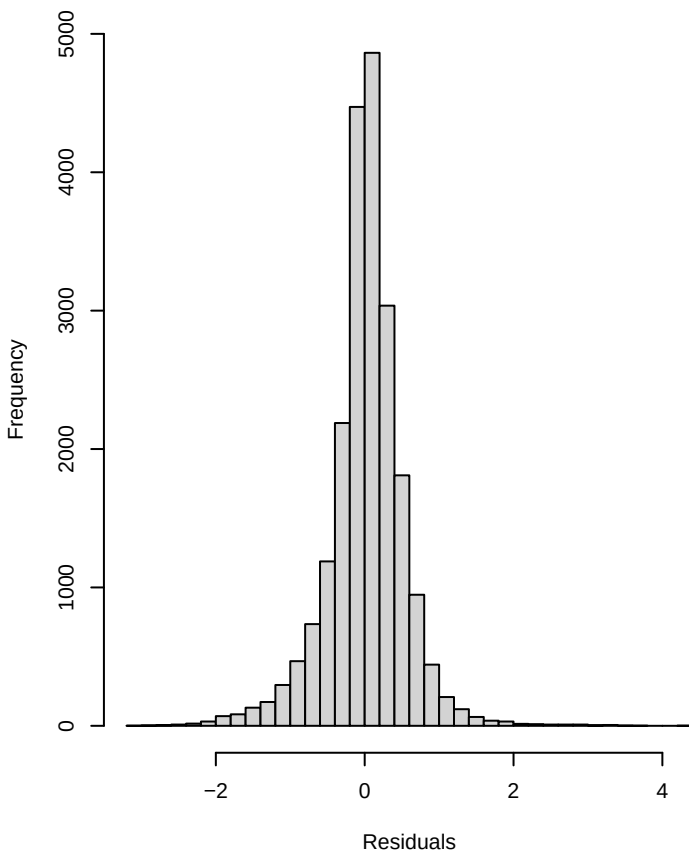
K_corr - Residual Distribution
