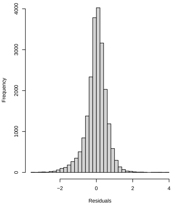
A_corr – Residual Distribution
