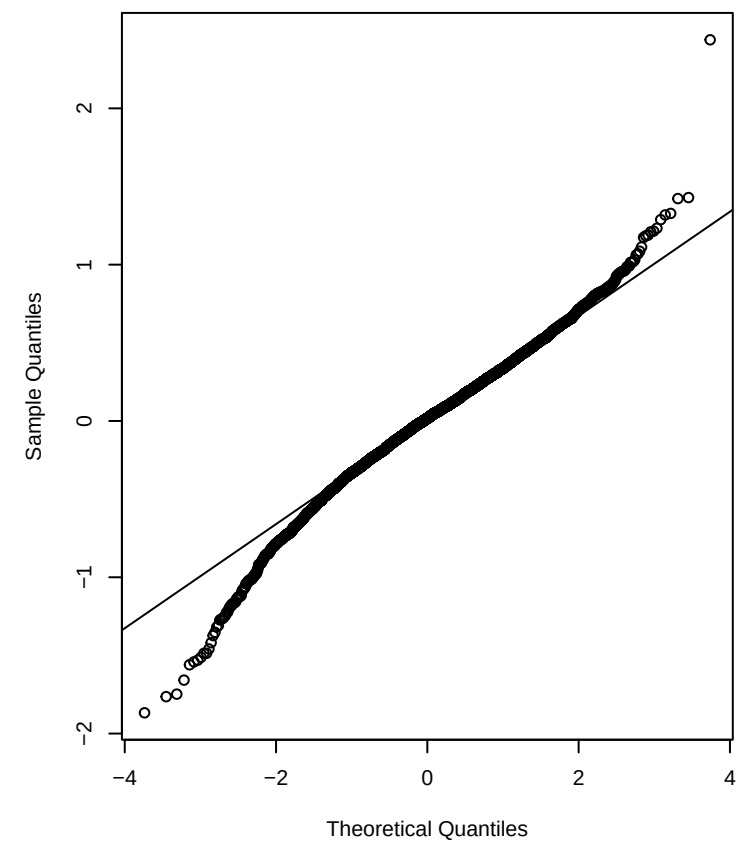
A_corr – Random Effects Q-Q
