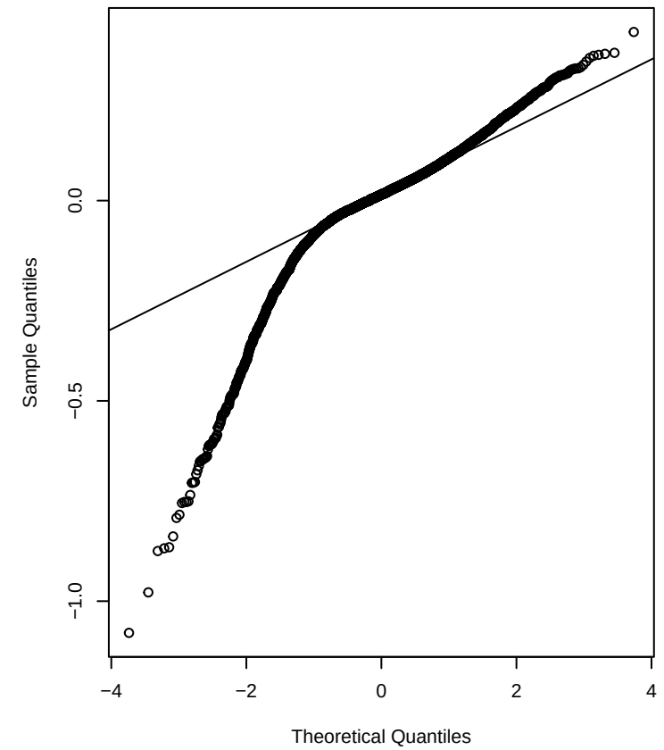
K_corr - Random Effects Q-Q
