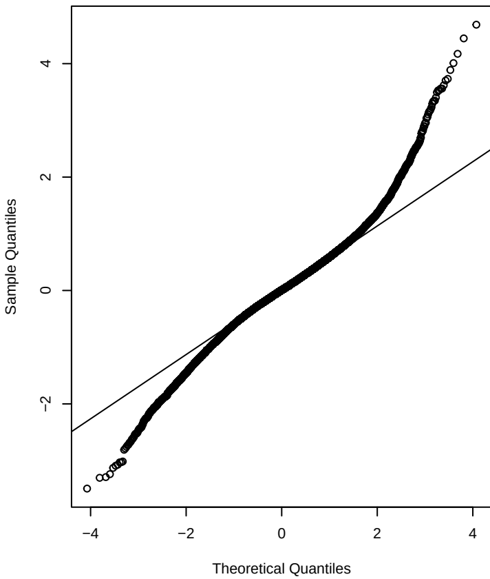
AC_corr_pearson – Q-Q Plot
