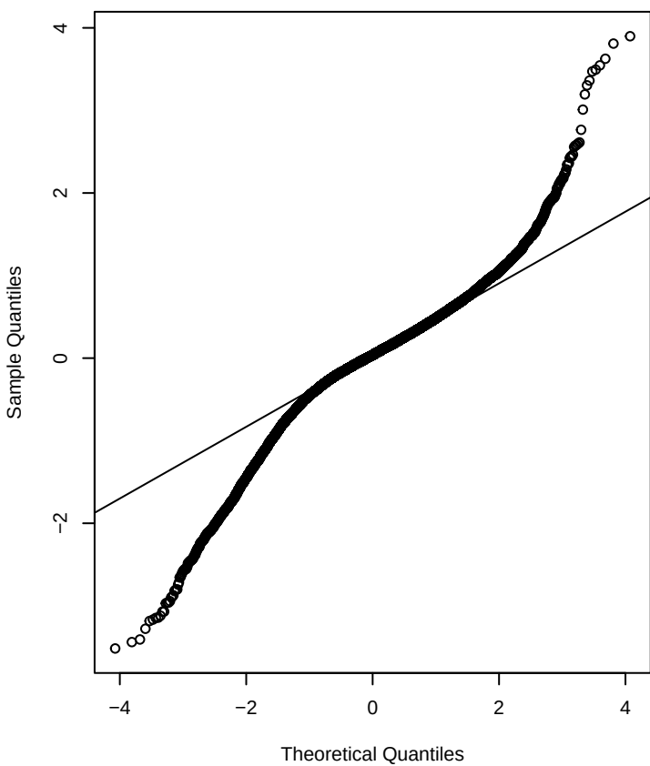
A_corr – Q-Q Plot
