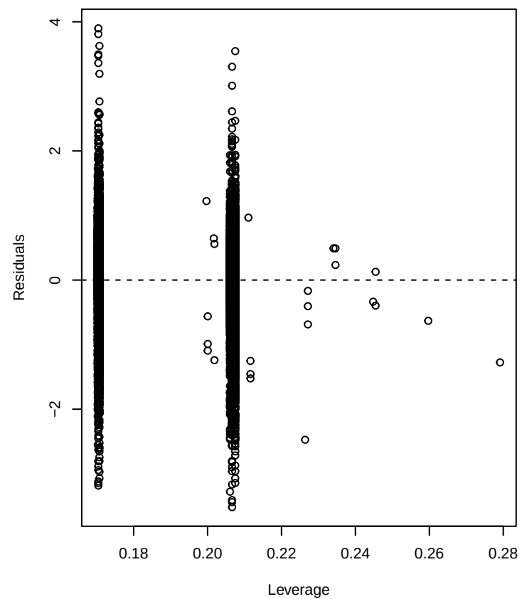
A_corr – Residuals vs Leverage
