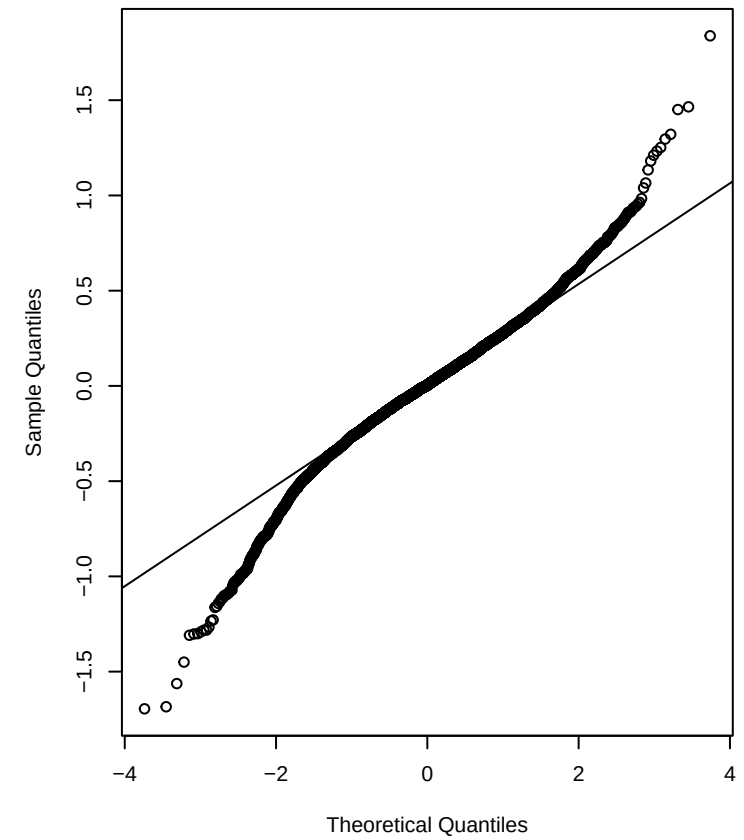
AC_corr_pearson – Random Effects Q-Q
