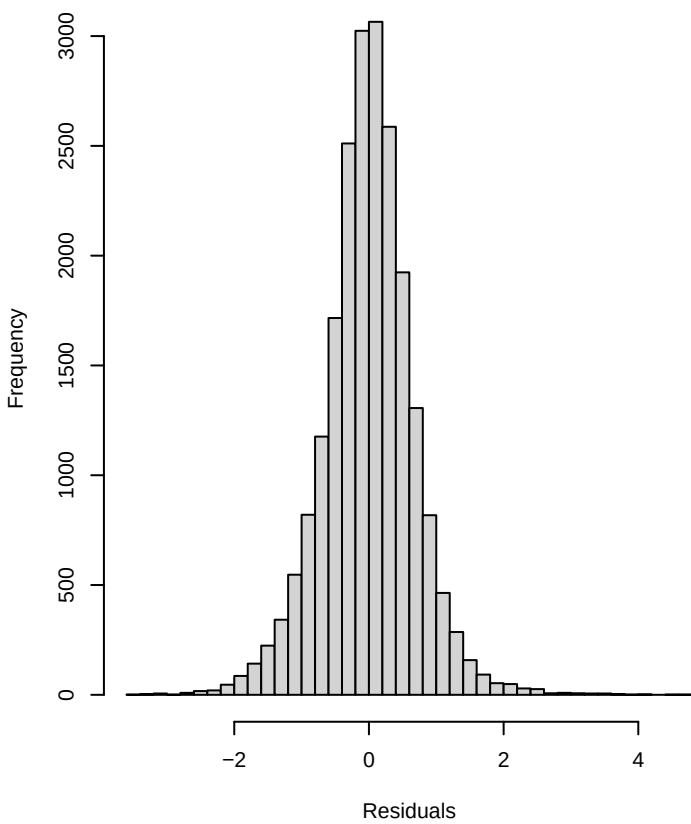
AC_corr_pearson – Residual Distribution
