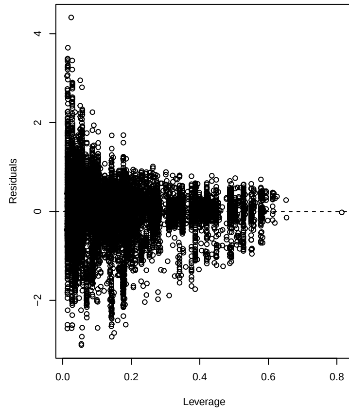
K_corr - Residuals vs Leverage
