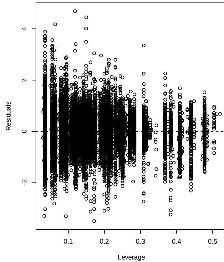
AC_corr_pearson – Residuals vs Leverage
