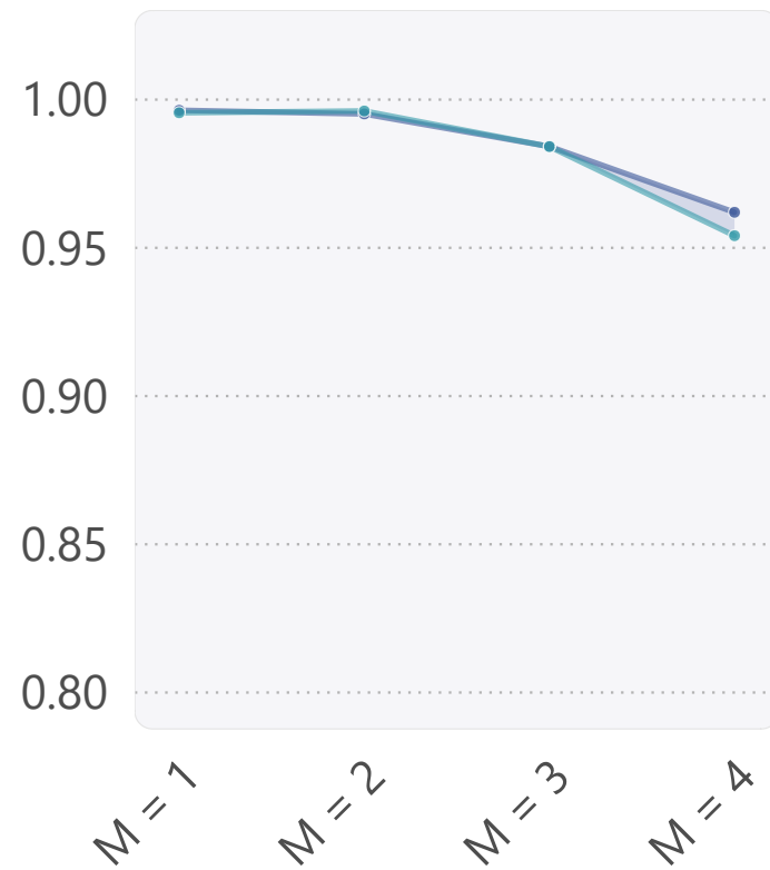
temporal (A)
