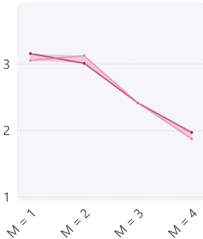
temporal (A)
