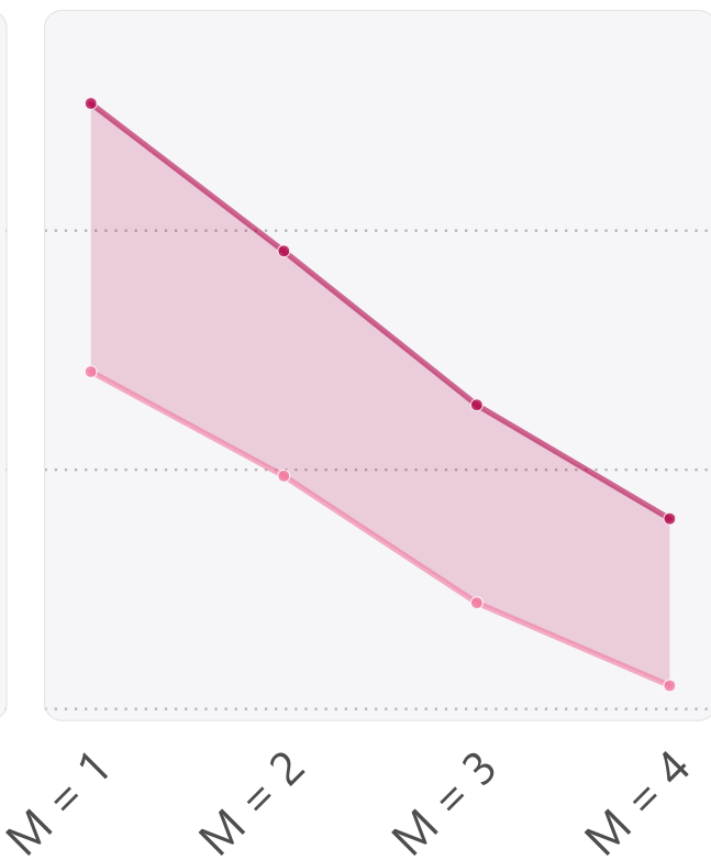
contemporaneous (K)
