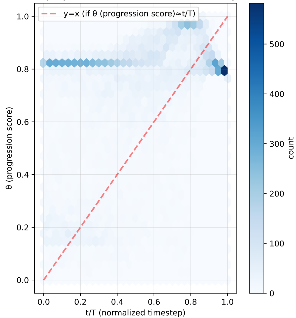
\theta (progression score) vs t/T Hexbin Density
