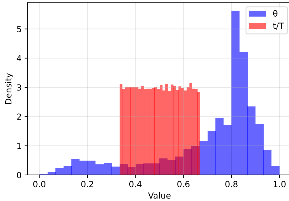
Mid (33-67%) (KS=0.7085, p=0.00e+00)
