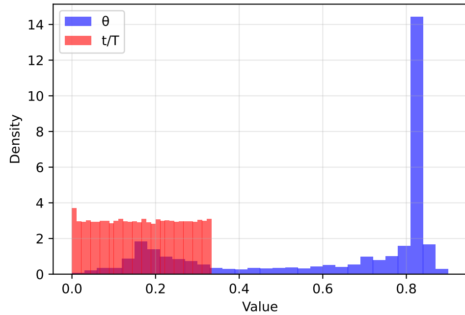
Early (0-33%) (KS=0.7544, p=0.00e+00)
