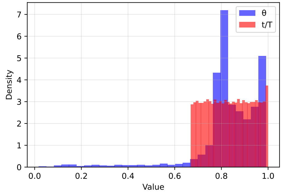
Late (67-100%) (KS=0.1851, p=2.00e-98)
