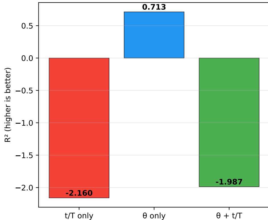
RUL Prediction R^2 (Downstream Transformer)
