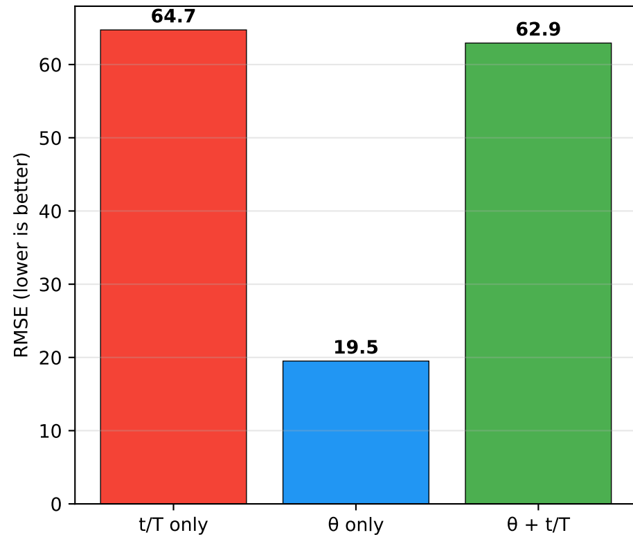
RUL Prediction RMSE (Downstream Transformer)
