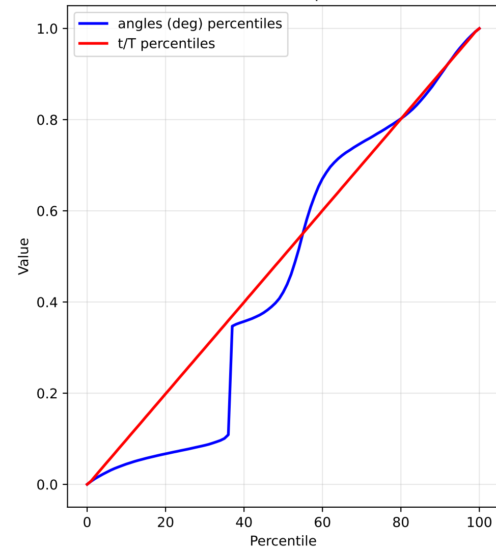
Percentile Comparison
