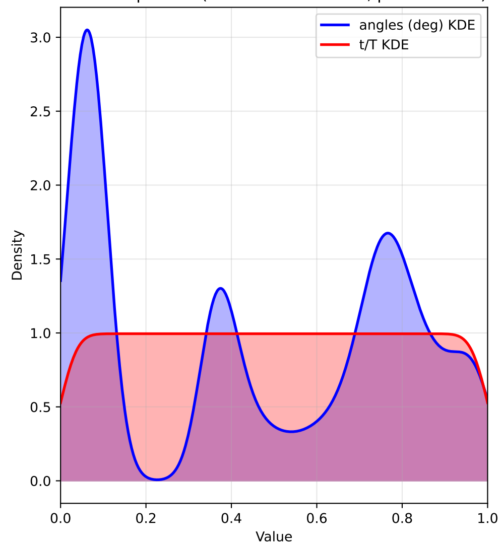
Distribution Statistics
