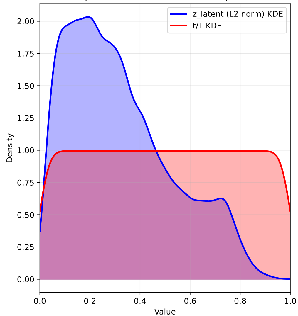
Distribution Statistics
