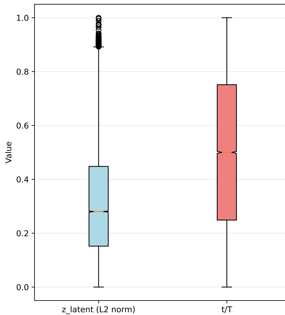
Distribution Statistics
