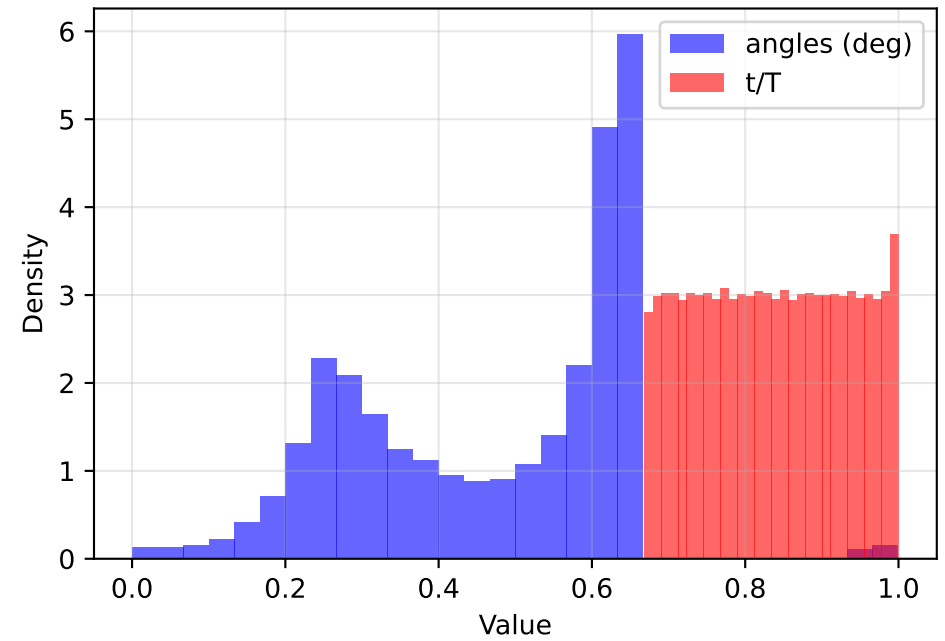
Late (67-100%) (KS=0.9909, p=0.00e+00)
