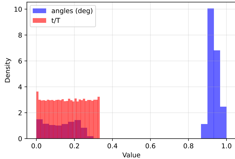
Early (0-33%) (KS=0.6815, p=0.00e+00)
