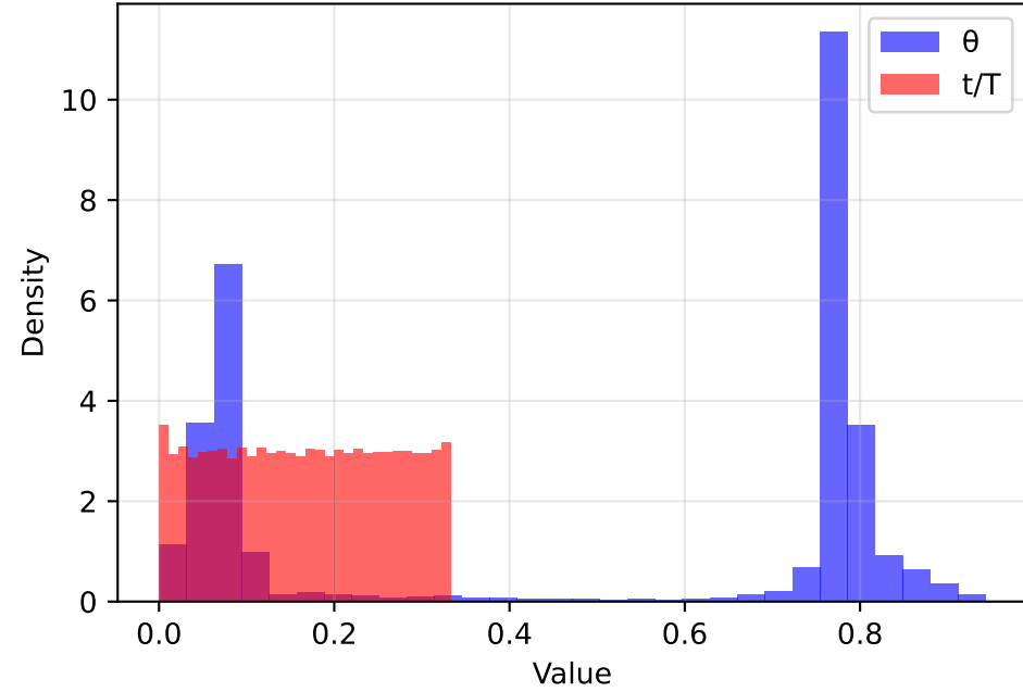
Early (0-33%) (KS=0.5838, p=0.00e+00)
