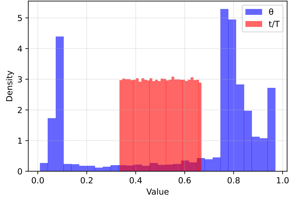
Mid (33-67%) (KS=0.6719, p=0.00e+00)
