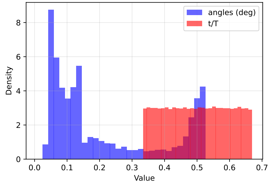
Mid (33-67%) (KS=0.7301, p=0.00e+00)
