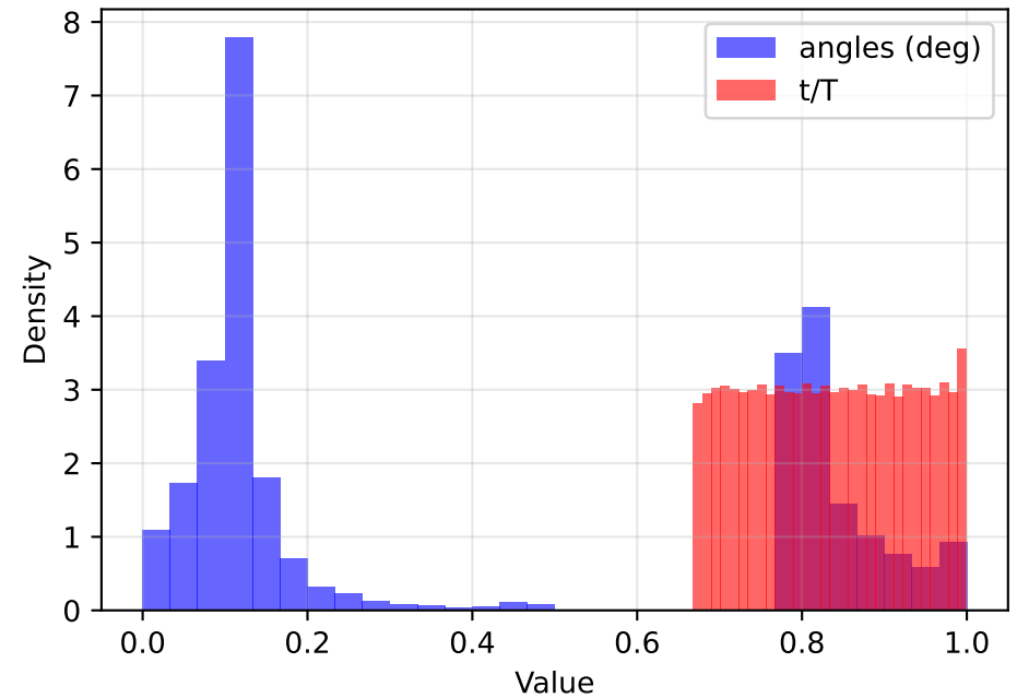
Late (67-100%) (KS=0.5876, p=0.00e+00)
