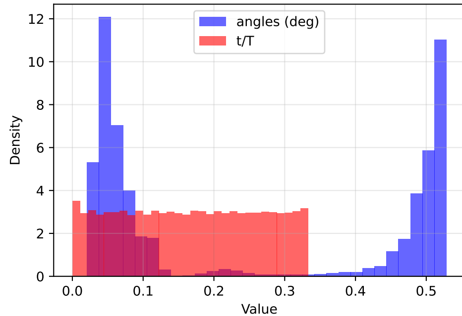
Early (0-33%) (KS=0.4264, p=0.00e+00)
