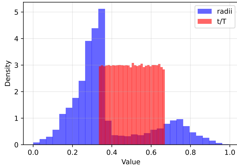
Mid (33-67%) (KS=0.6150, p=0.00e+00)
