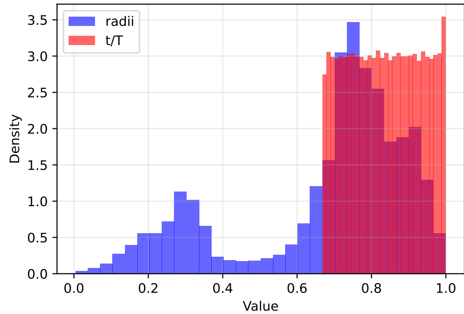
Late (67-100%) (KS=0.3022, p=0.00e+00)
