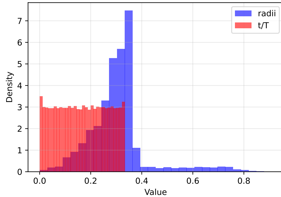
Early (0-33%) (KS=0.5040, p=0.00e+00)
