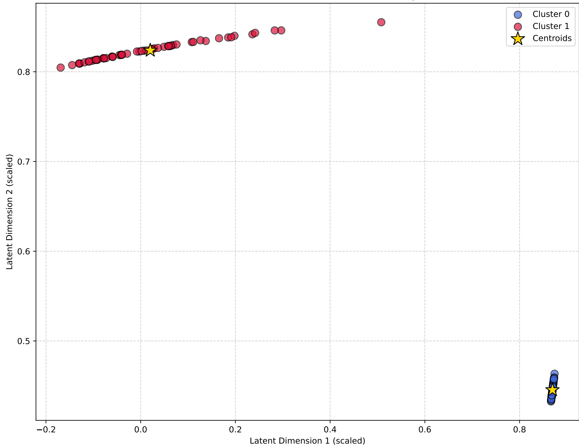
k-means (k=2) on Mean of Last 10 Latent Vectors per Unit
