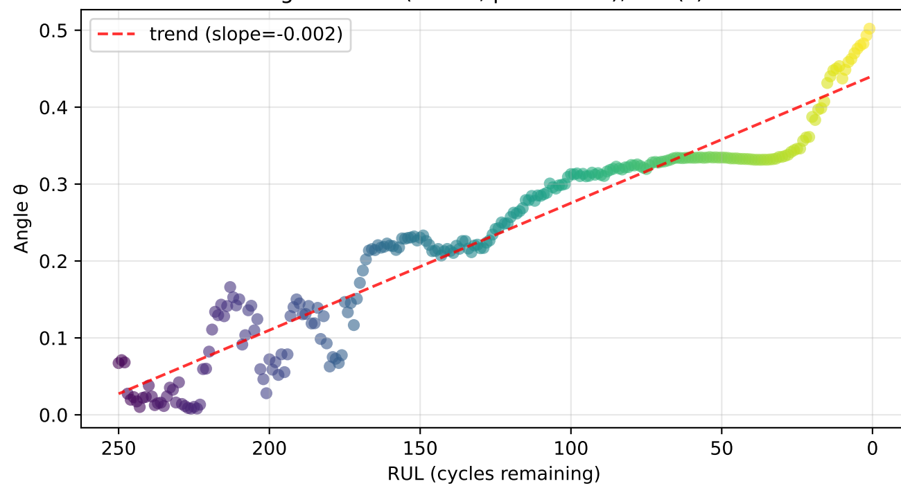
Angle vs RUL (Unit 1, \rho = -0.978 ), \dim(z)=4
