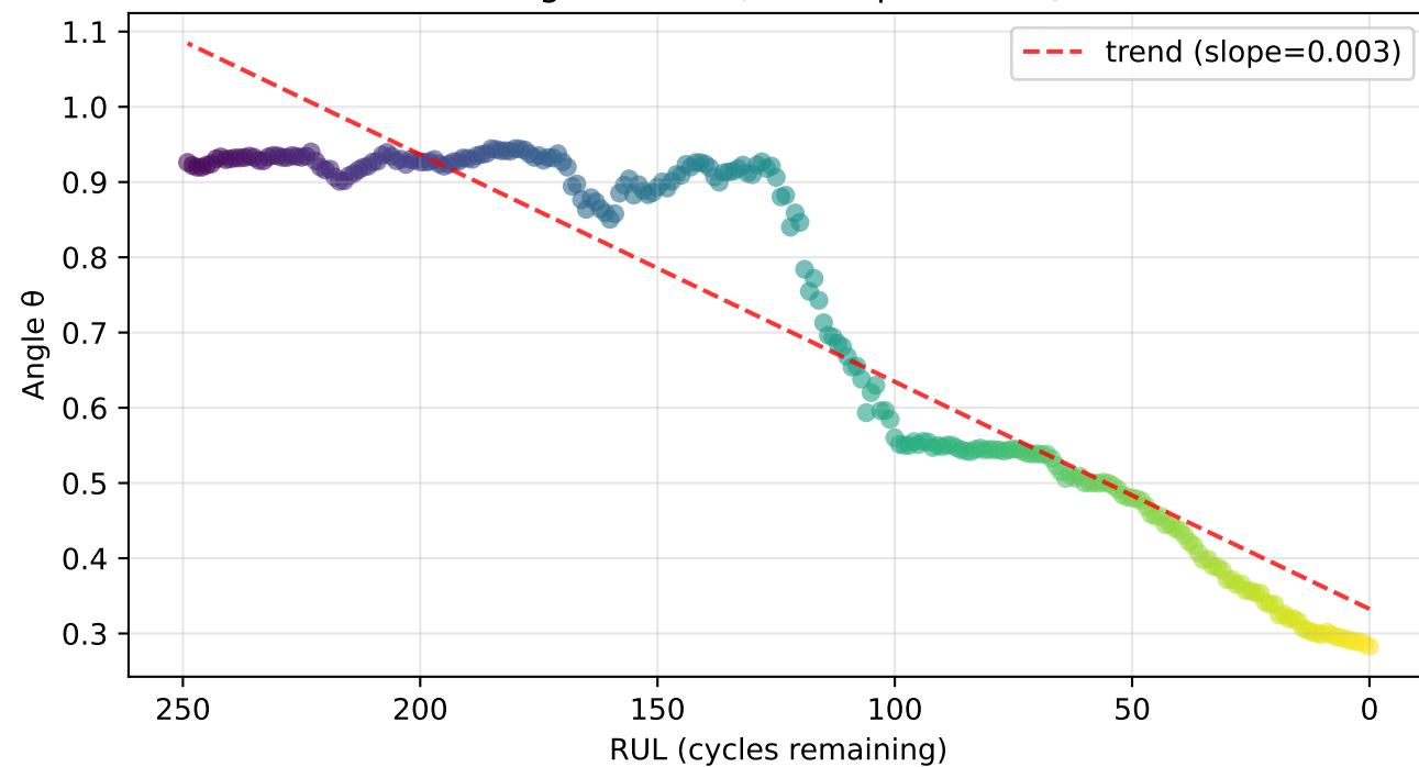
Angle vs RUL (Unit 1, \rho = 0.931 )
