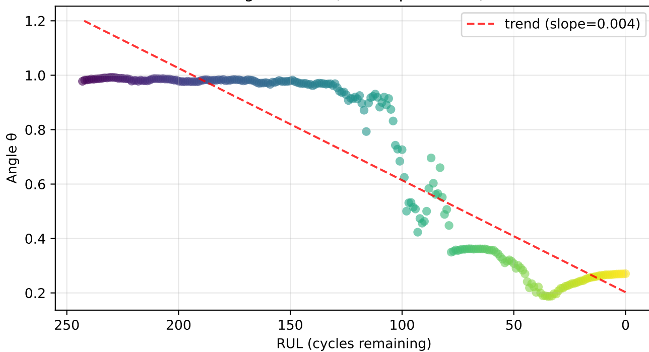
Angle vs RUL (Unit 2, \rho = 0.963 )
