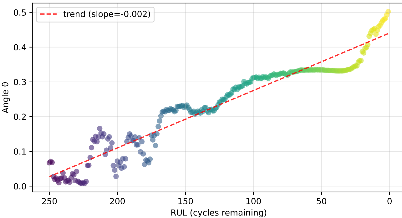
Angle vs RUL (Unit 1, \rho = -0.978 ), \dim(z)=4
