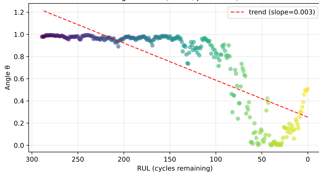
Angle vs RUL (Unit 2, \rho = 0.885 )
