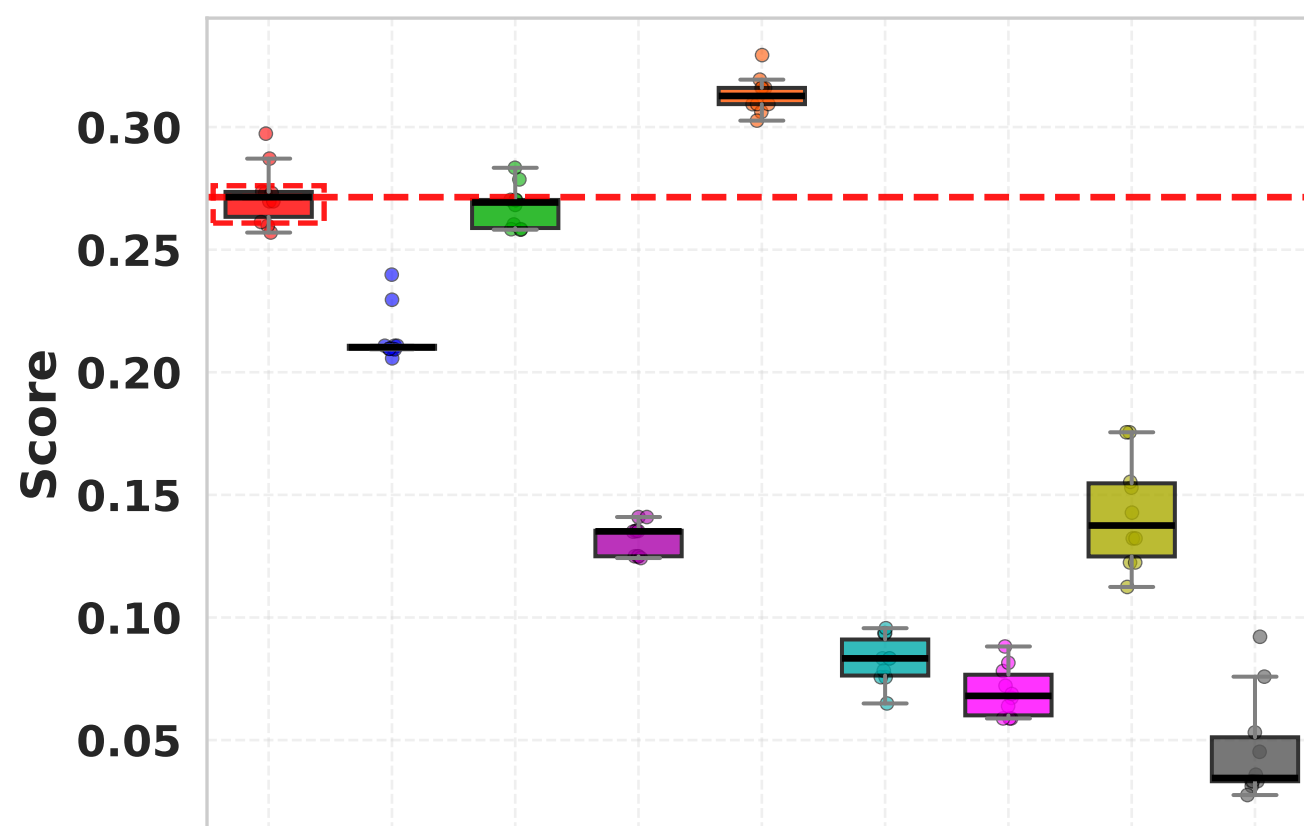
Silhouette Score
