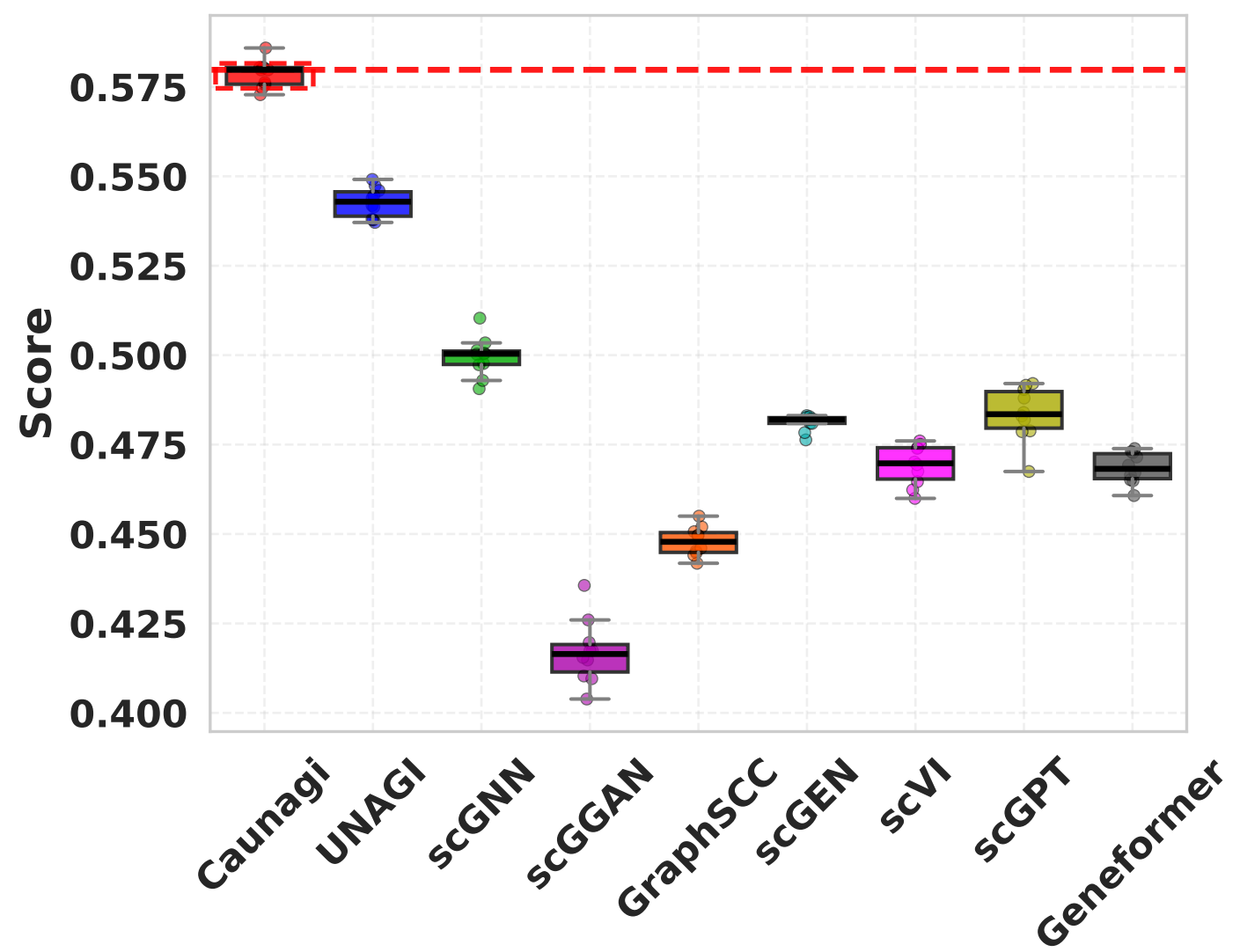
Overall SCIB
