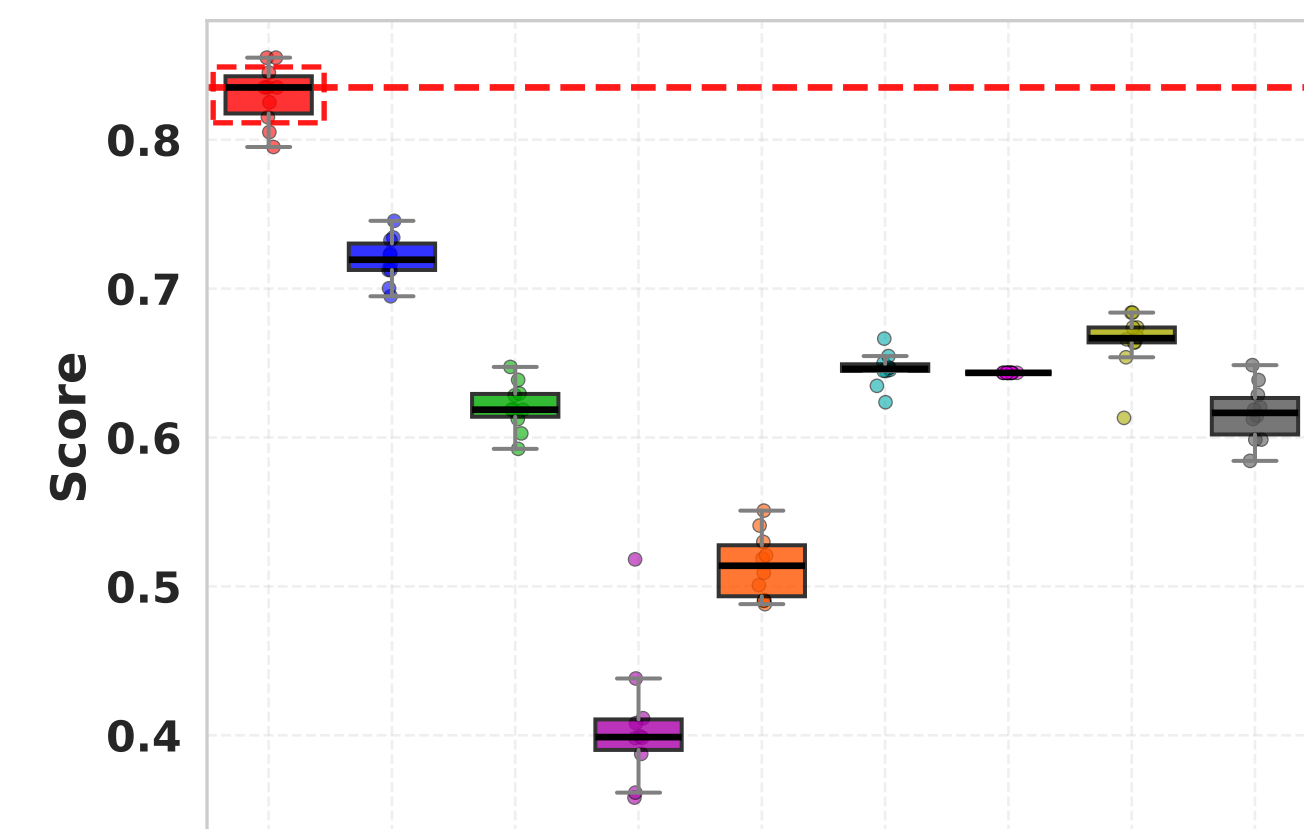
ARI
