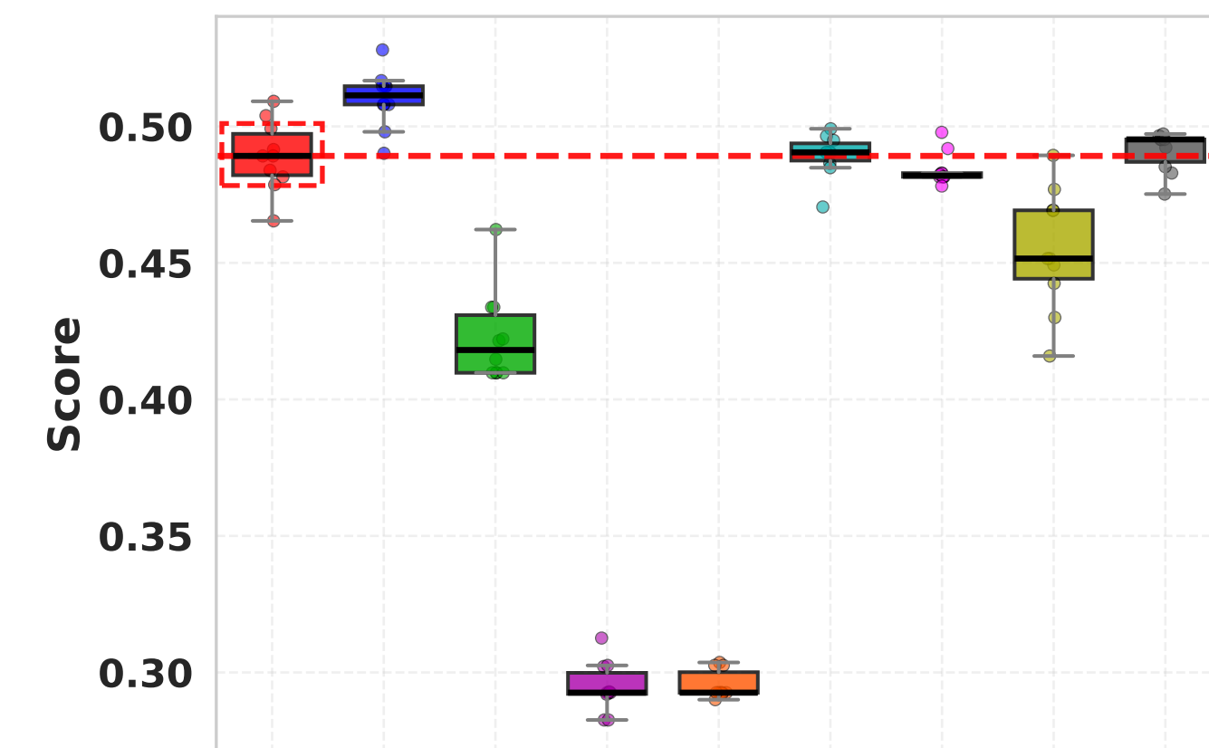
Isolated ASW
