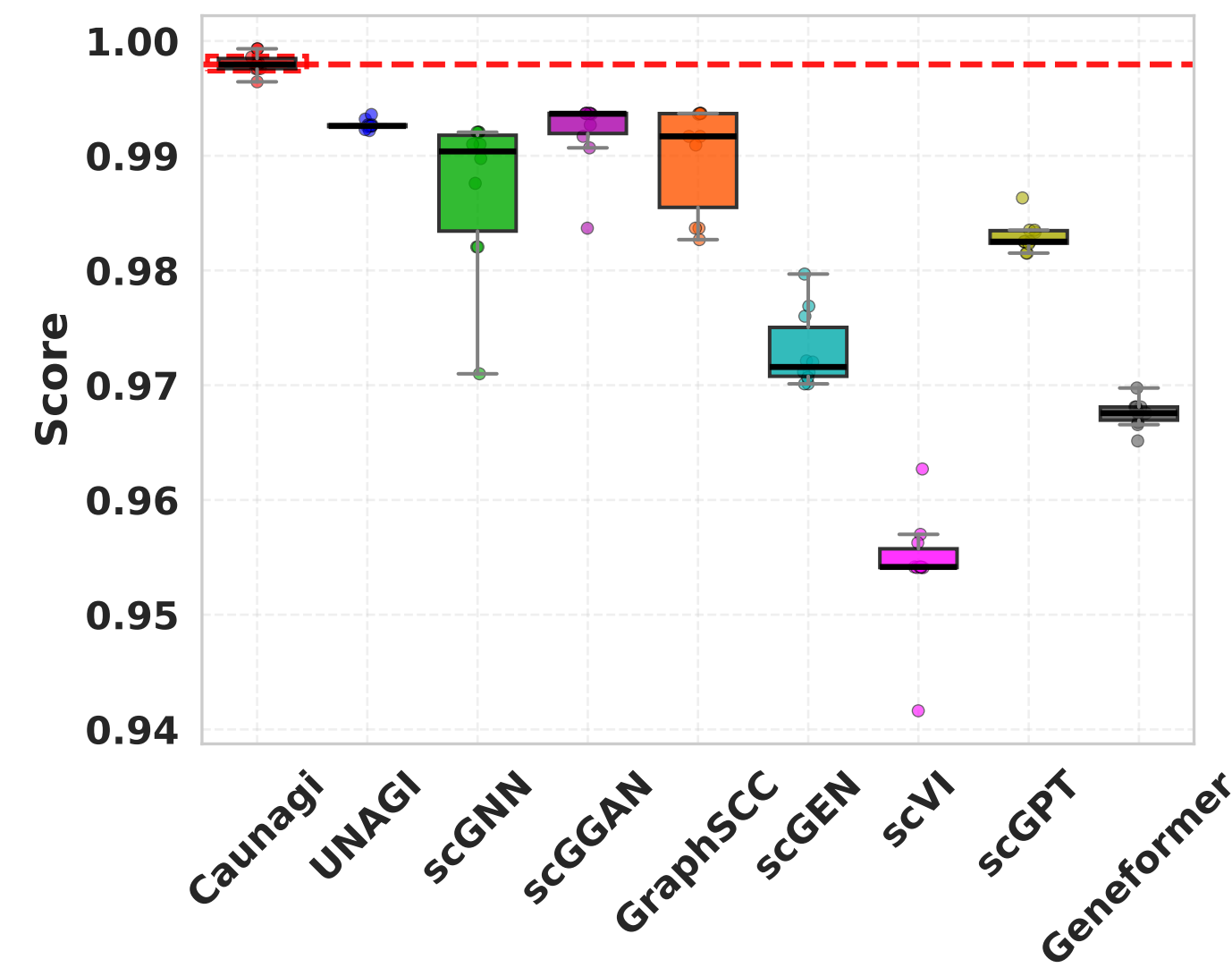
Clisi_graph
