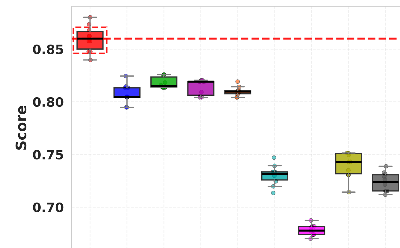
Label score
