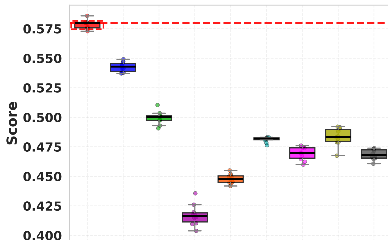
Overall SCIB
