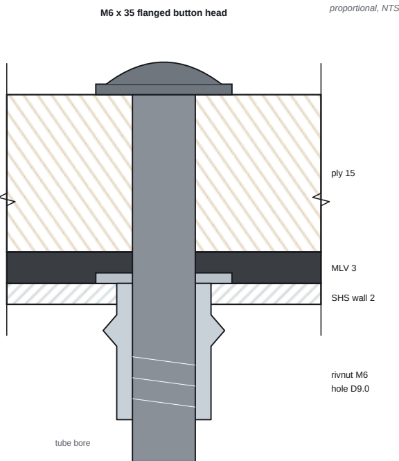
F M6 RIVNUT PANEL FIXING
