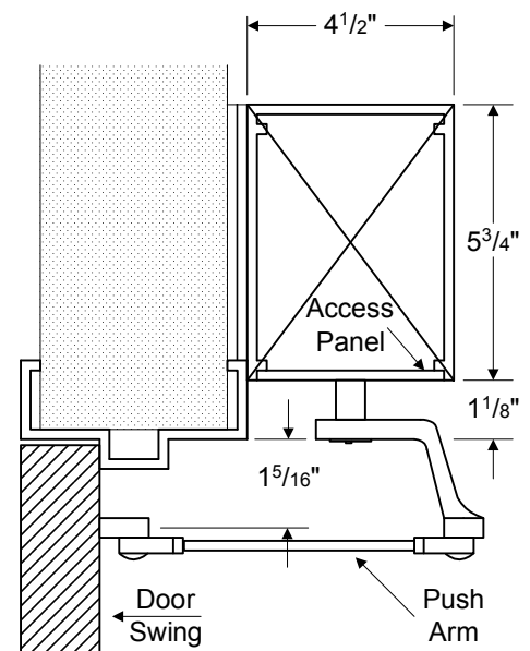
Vertical Section ③
