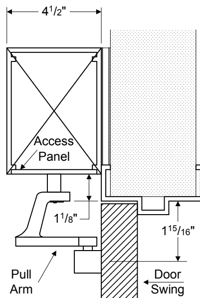
② Vertical Section
