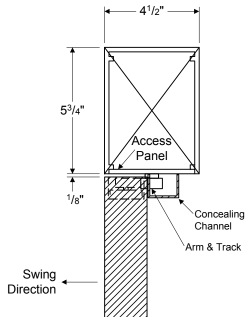
② Vertical Section
