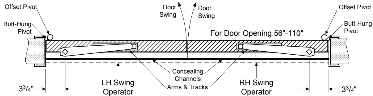
① Horizontal Section
