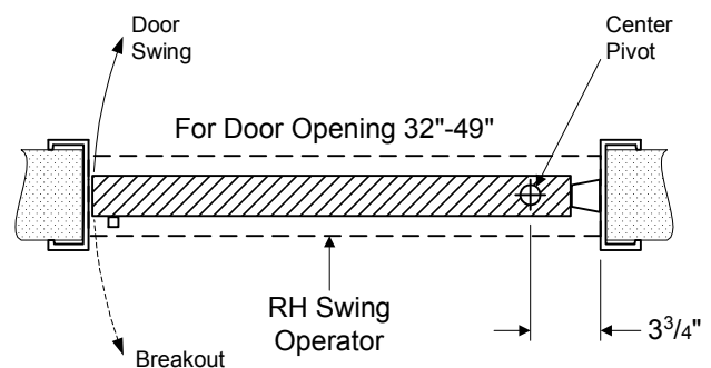
① Horizontal Section
