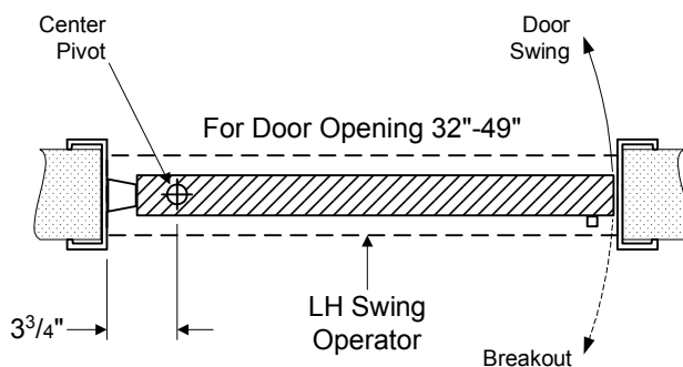
① Horizontal Section
