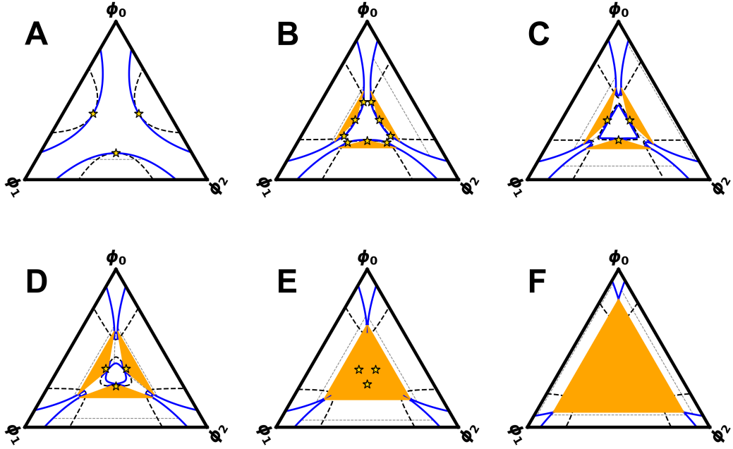
Figure 18: Phase diagram for different values of \chi . The orange areas are the three-phase regions, the binodal is shown in blue, the spinodal is the thick dashed line and the critical points are the gold stars and the tie-lines are the thin striped lines. The three-phase regions are shown as shaded areas. (A) \chi = 2.4 , (B) \chi = 2.65 , (C) \chi = 8/3 , (D) \chi = 2.7 , (E) \chi = 2.746 , (F) \chi = 3.0 .
