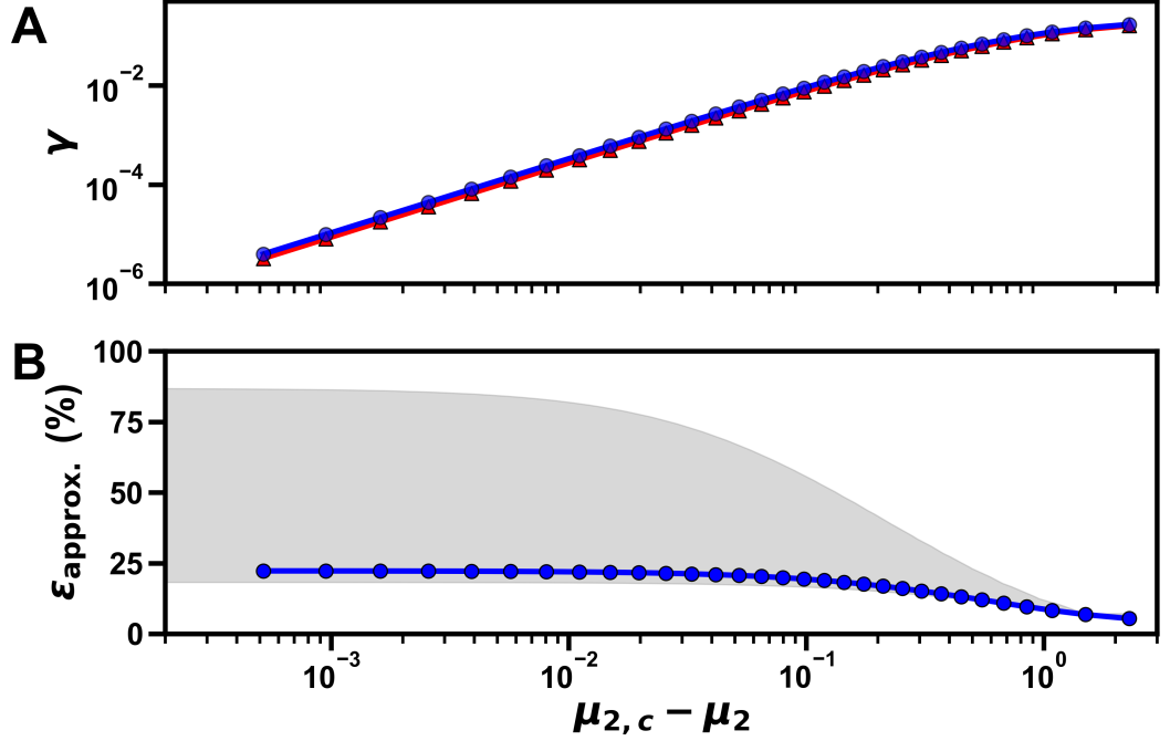
Figure 9: (A) Exact (red) and approximate (blue) surface tension for \chi_{01} = 2.5 , \chi_{02} = 1.5 , \chi_{12} = 1.4 as a function of the chemical potential. (B) Relative error \epsilon_{\text{approx}} = (\gamma_{\text{approx}} - \gamma_{\text{exact}})/\gamma_{\text{exact}} , where the blue data points correspond to the same parameters as in (A) and the gray area indicates the range of errors obtained for the other interaction parameters in Eq. (18).
