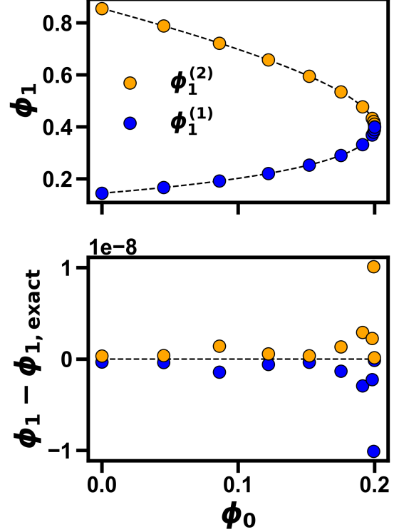
Figure 19: Top: Binodal curve for the symmetric ternary system with \chi_{01} = \chi_{02} = 1.5 and \chi_{12} = 2.5 . The dashed line shows the analytical solution from Eq. 45, while the blue and orange points show the results obtained with our algorithm. Bottom: The residual between the analytical and numerical results is negligible.
