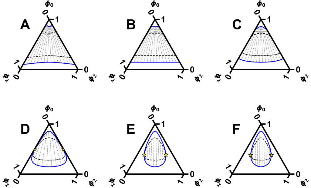
Figure 19: Phase diagram for varying \chi = -5 and varying \delta . (A) \delta = -0.5 , (B) \delta = 0.0 , (C) \delta = 0.5 , (D) \delta = 1.1 , (E) \delta = 10.0 and (F) \delta = 60.0 .
