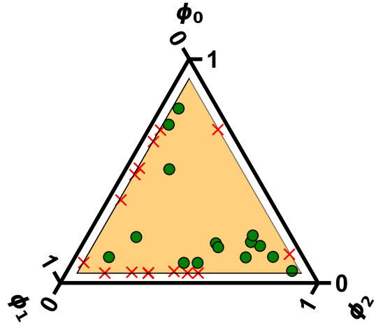
Figure 12: Comparison of the coexistence compositions obtained from our algorithm and the flory package for points in the three phase region (orange area). The green points correspond to correct predictions from the flory package, while the red crosses indicate cases where two phase compositions were found yielding a higher free energy.
