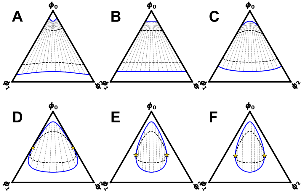
Figure 15: Phase diagram for varying \delta
