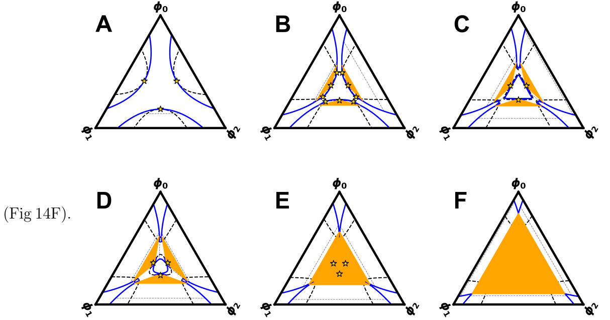
Figure 14: Phase diagram for different values of \chi . The orange areas are the three-phase regions, the binodal is shown in blue, the spinodal is the thick dashed line, and the critical points are the gold stars and the tie-lines are the thin striped lines. The three-phase regions are shown as shaded areas. (A) \chi = 2.4 , (B) \chi = 2.65 , (C) \chi = 8/3 , (D) \chi = 2.7 , (E) \chi = 2.746 , (F) \chi = 3.0 .
