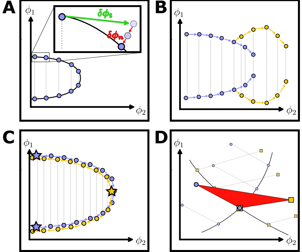
Figure 10: Schematic illustration of the main steps and characteristic events in the algorithm, shown in the \phi_1 - \phi_2 phase space. (A) Successive tangential (green arrow) and projection (red arrow) steps; the projection step may need to be repeated. (B) Branching event: an initial binodal section (blue) splits into a second section (orange) when the Jacobian becomes degenerate. (C) Duplicate binodal sections obtained when tracing is initiated either from the dilute limit (blue points) or from the critical point (orange points). The stars denote the initial points of the tracing processes. (D) The crossing of two binodal branches indicates a three-phase region (red triangle).
