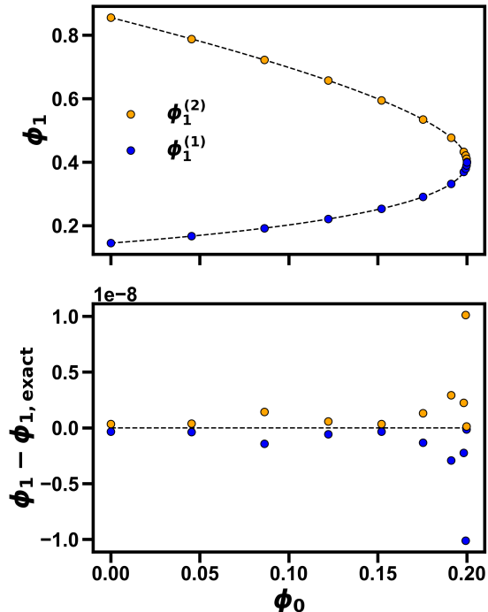
Figure 13: Binodal curve for the symmetric ternary system with \chi_{01} = \chi_{02} = 1.5 and \chi_{12} = 2.5 . The dashed line shows the analytical solution from Eq. 35, and the blue and orange points show the results from our algorithm.
