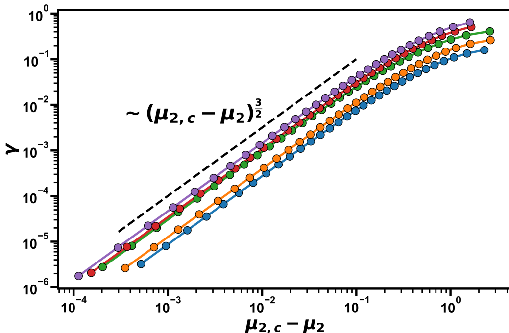
Figure 7: Surface tension as a function of the chemical potential difference \mu_{2,c} - \mu_2 for various interaction parameters (colored lines) in the range specified by Eq. (17). The surface tension exhibits a power-law scaling \gamma \sim (\mu_{2,c} - \mu_2)^{3/2} close to criticality (dashed line).
