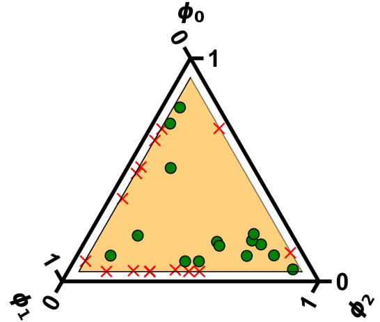
Figure 18: Comparison of three phase coexistence compositions obtained from our algorithm and the flory package for points in the three-phase region (orange area). The green points correspond to correct predictions from the flory package, while the red crosses indicate cases where two-phase compositions were found that yield a slightly higher free energy. Add legend and fill entire textwidth
