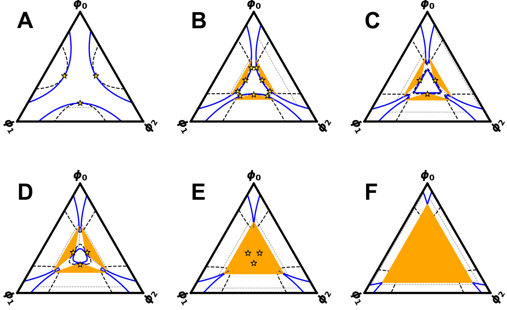
Figure 20: Phase diagram for different values of \chi . The orange triangles are the three-phase regions, the binodal is shown in blue, the spinodal is the thick dashed line and the critical points are the gold stars and the tie-lines are the thin striped lines. (A) \chi = 2.4 , (B) \chi = 2.65 , (C) \chi = 8/3 , (D) \chi = 2.7 , (E) \chi = 2.746 , (F) \chi = 3.0 . Maybe add legend
