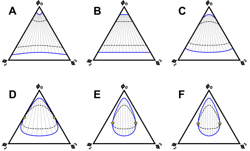
Figure 21: Phase diagram for \chi = -5 and varying \delta \in [-0.5, 60.0] . Blue line denote binodals, black dashed lines denote spinodal. (A) \delta = -0.5 , (B) \delta = 0.0 , (C) \delta = 0.5 , (D) \delta = 1.1 , (E) \delta = 10.0 and (F) \delta = 60.0 .
