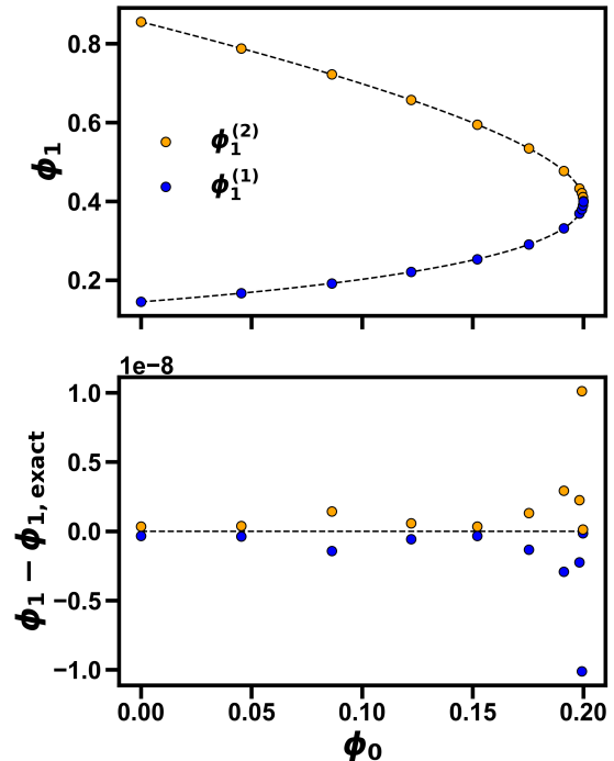
Figure 19: Binodal curve for the symmetric ternary system with \chi_{01} = \chi_{02} = 1.5 and \chi_{12} = 2.5 . The dashed line shows the analytical solution from Eq. 43 and the blue and orange points show the results from our algorithm.
