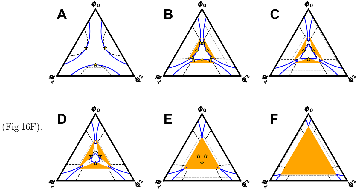
Figure 16: Phase diagram for different values of \chi . The orange areas are the three-phase regions, the binodal is shown in blue, the spinodal is the thick dashed line, and the critical points are the gold stars and the tie-lines are the thin striped lines. The three-phase regions are shown as shaded areas. (A) \chi = 2.4 , (B) \chi = 2.65 , (C) \chi = 8/3 , (D) \chi = 2.7 , (E) \chi = 2.746 , (F) \chi = 3.0 .
