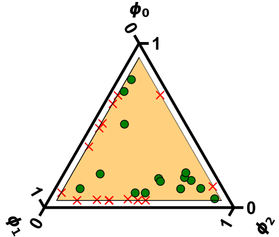
Figure 14: Comparison of the coexistence compositions obtained from our algorithm and the flory package for points in the three phase region (orange area). The green points correspond to correct predictions from the flory package, while the red crosses indicate cases where two phase compositions were found yielding a higher free energy.
