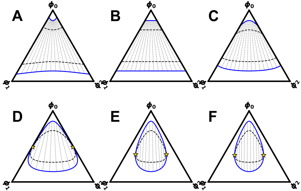
Figure 17: Phase diagram for varying \delta
