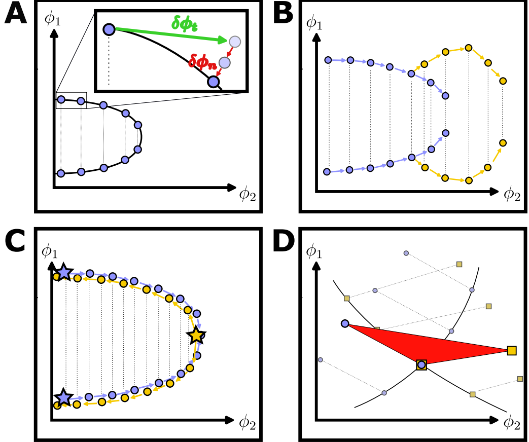
Figure 12: Schematic illustration of the main steps and characteristic events in the algorithm, shown in the \phi_1 - \phi_2 phase space. (A) Successive tangential (green arrow) and projection (red arrow) steps; the projection step may need to be repeated. (B) Branching event: an initial binodal section (blue) splits into a second section (orange) when the Jacobian becomes degenerate. (C) Duplicate binodal sections obtained when tracing is initiated either from the dilute limit (blue points) or from the critical point (orange points). The stars denote the initial points of the tracing processes. (D) The crossing of two binodal branches indicates a three-phase region (red triangle).
