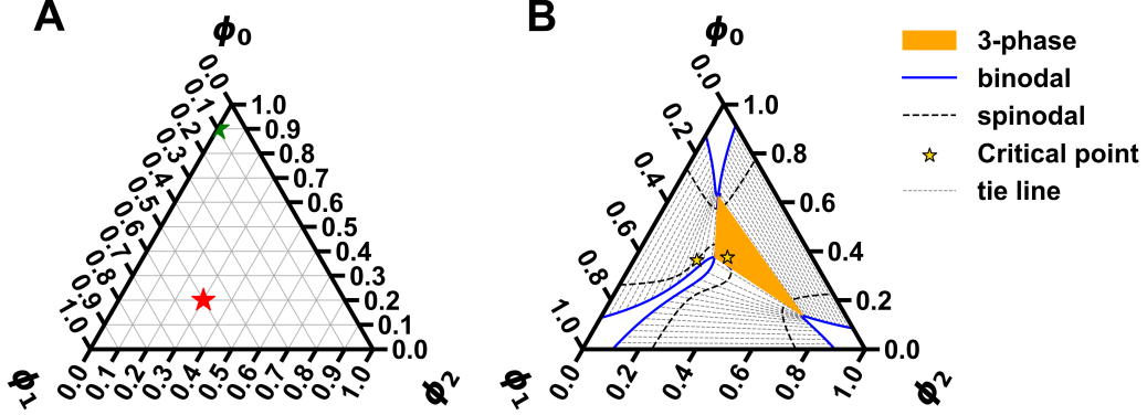
Figure 17: (A) Ternary diagram, with axes \phi_0 on the right diagonal, \phi_1 on the left diagonal and \phi_2 on the horizontal axis. The red star is at (\phi_0 \phi_1 \phi_2)^T = (0.2 \ 0.5 \ 0.3)^T and the green star is at (\phi_0 \phi_1 \phi_2)^T = (0.9 \ 0.1 \ 0.0)^T . Note that the sum of the three volume fractions is always 1.
