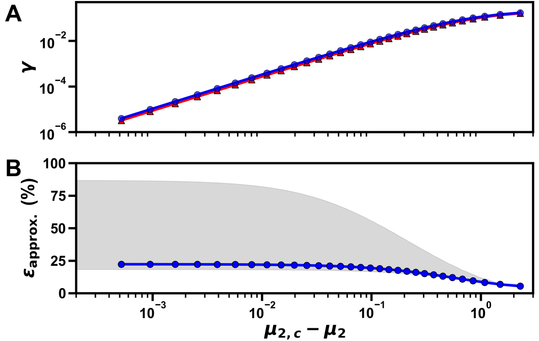
Figure 9: (A) Exact (red) and approximate (blue) surface tension for \chi_{01} = 1.4 , \chi_{02} = 1.5 , \chi_{12} = 2.5 as a function of the chemical potential. (B) Relative error \epsilon_{\text{approx}} = (\gamma_{\text{approx}} - \gamma_{\text{exact}})/\gamma_{\text{exact}} , where the blue data points correspond to the same parameters as in (A) and the gray area indicates the range of errors obtained for the other interaction parameters in Eq. (20).
