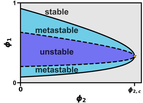
Figure 2: Phase diagram of ternary system showing the binodal (solid black line), spinodal (dashed black line), and the regions of stability, metastability and instability of the homogenous state as well as the critical point (gold star).
