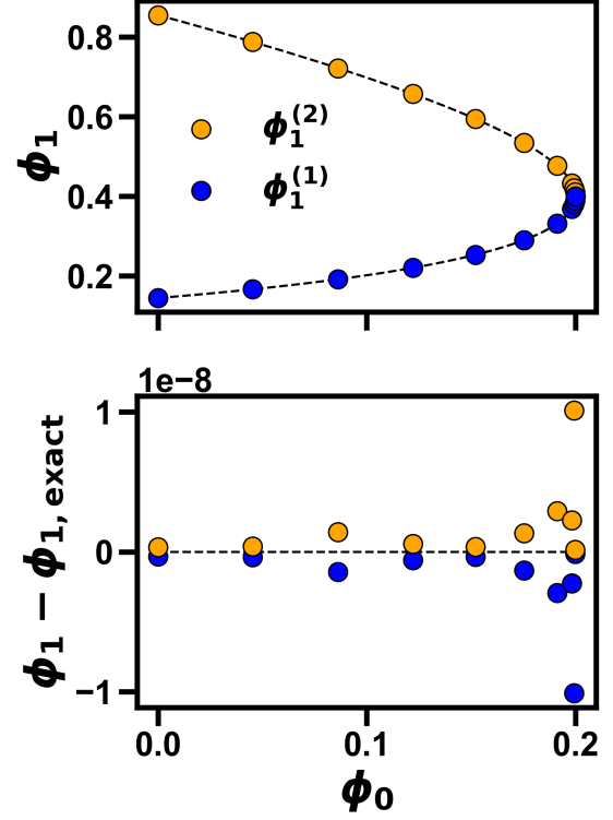
Figure 19: Top: Binodal curve for the symmetric ternary system with \chi_{01} = \chi_{02} = 1.5 and \chi_{12} = 2.5 . The dashed line shows the analytical solution from Eq. 44, while the blue and orange points show the results obtained with our algorithm. Bottom: The residual between the analytical and numerical results is negligible.
