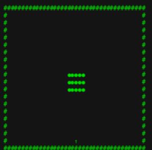
DNMS Task
