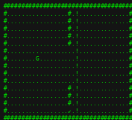
Shuttle Box
