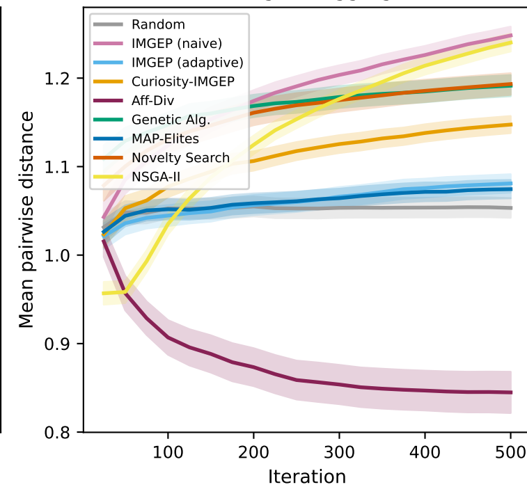
(h) All targets (aggregated)
