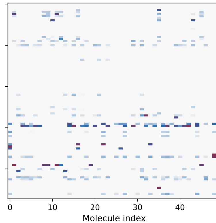
Random
