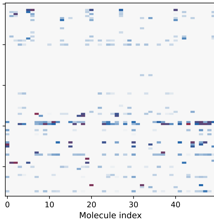
MAP-Elites
