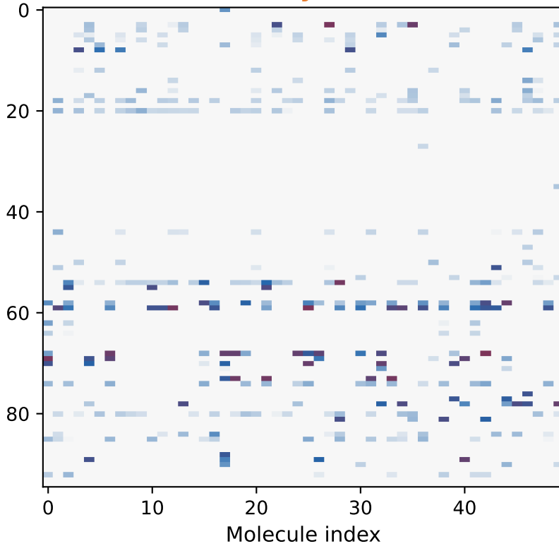
Curiosity-IMGEP
