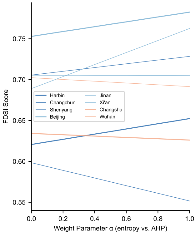
(a) FDSI Sensitivity to \alpha
