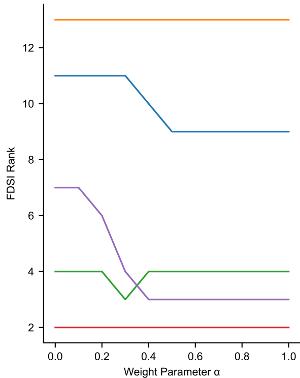
(b) Rank Stability vs. \alpha
